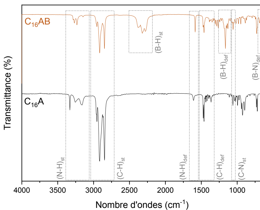
Figure 4 : Spectres IRTF de C_{16}A et de C_{16}AB
