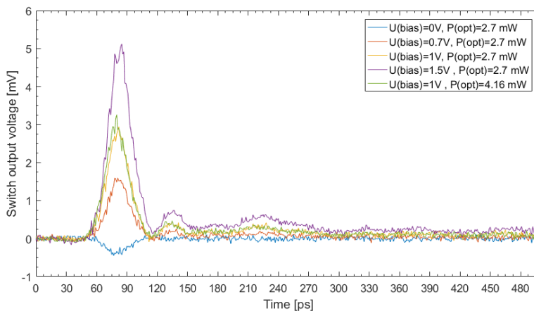
Figure 2-27 Measured pulses with the fast sampling oscilloscope for SA2-2 switch
