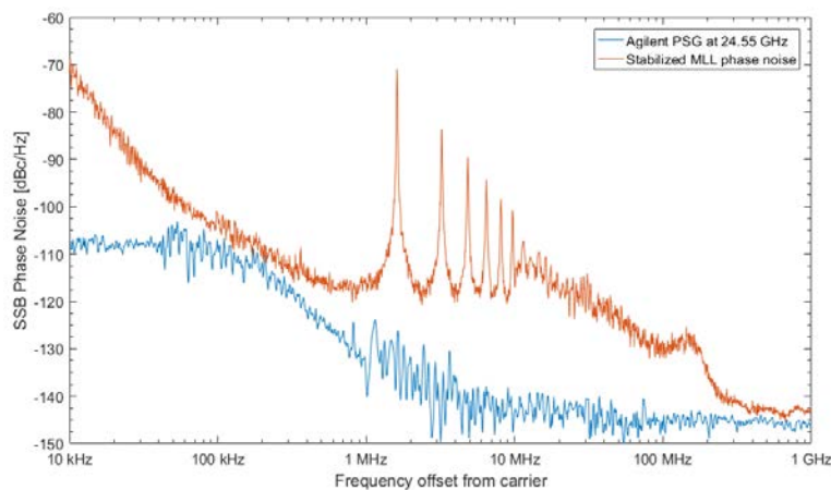
Figure 4-27 Comparison of the PSG phase noise and the MLL phase noise
