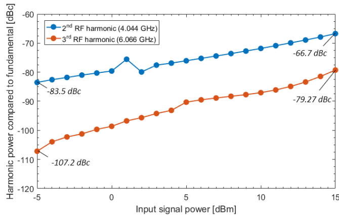
Figure 4-32 Power levels of the input RF signal harmonics at the generator output. f_{RF} = 2.022 GHz, P_{RF} = 15 dBm
