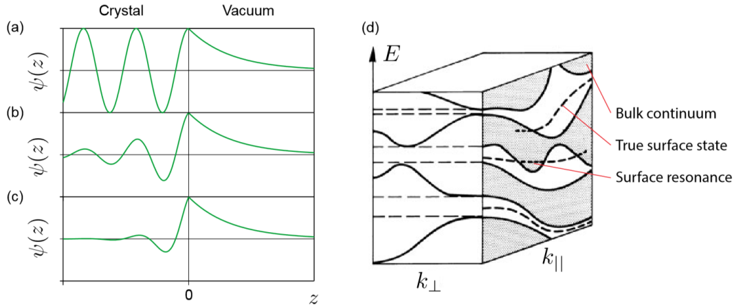
FIGURE 1.2: Electronic wavefunction at the sample surface for a bulk band (a), a surface resonance (b) and a surface state (c). z < 0 corresponds to the solid and z > 0 is the vacuum [14]. (d) Schematics of bulk-surface wavefunction overlap in a three dimensional band structure [21]. Solid lines correspond to bulk bands, shaded regions represent the projected bulk continuum states while white areas are band gaps. Surface solutions which exist within the band gaps and do not degenerate with the bulk continuum are true surface states, otherwise they are described as surface resonances.
