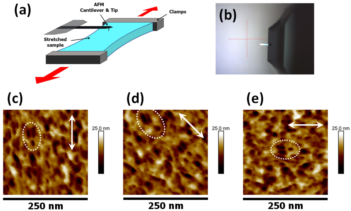
Figure 4.5. (a) Schematic of stretching for imaging of PDMS under mechanical stress, (b) OM micrograph of the top of an AFM cantilever ( \mu Masch) in close proximity (about 20 \mu m) above the stretched PDMS surface, (c–e) AFM images of free sample surface taken at exactly the same location at different scanning angles, i.e., 0°, 45°, and 90°. The scanning area is 250 \times 250 nm 2 . White arrows indicate the direction of sample elongation, white dashed circles show the same spot in all the images.
