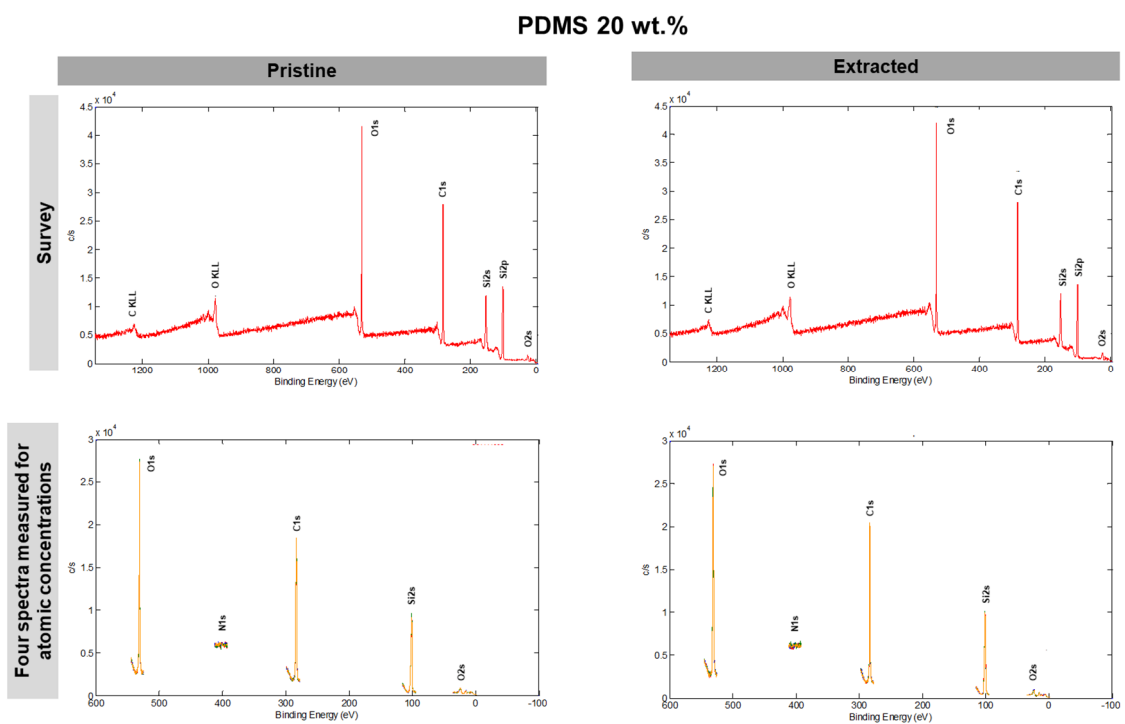
Figure S6. XPS survey spectra and four element spectra of O1s, N1s, C1s, Si2p, O2s regions for pristine and extracted PDMS with 20 wt.% of the cross-linker
