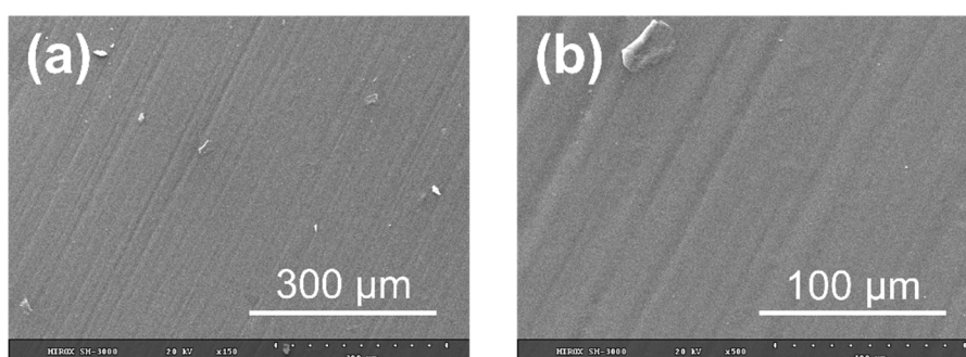
Figure 3.12. Representative SEM images of the flat-like LSR samples of Shore A stiffness 34 with a scale bar of (a) 300\text{ }\mu\text{m} and (b) 100\text{ }\mu\text{m} .
