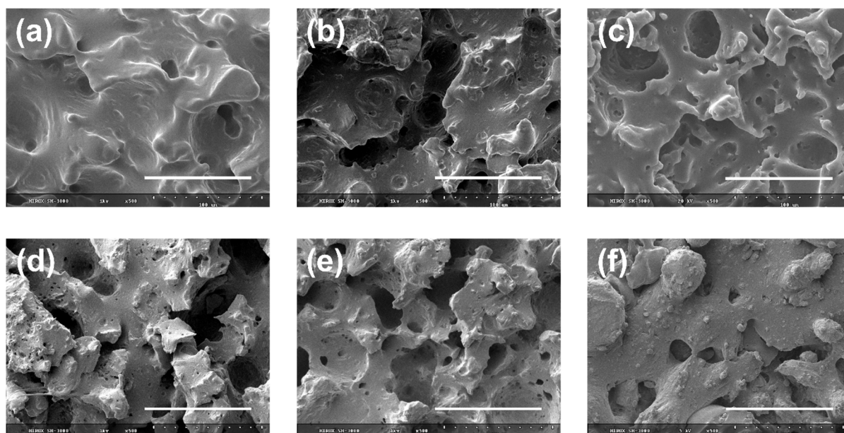
Figure 3.11. Representative SEM images of the textured LSR samples of varied Shore A stiffness: (a) 9, (b) 21, (c) 34, (d) 59, (e) 72. (f) SEM image of the superhydrophobic foil used as print surface. The scale bars represent 100 \mu\text{m} .
