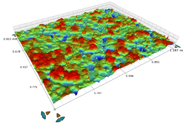
Figure 3.16. Topography of the textured LSR surface of 59 Shore A stiffness as reconstructed using the Vision software (mean roughness S_a = 19.9 \mu m , rms roughness S_q = 25.0 \mu m )
