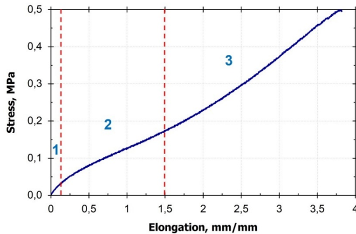
Figure 2.17. Representative stress-strain curve of the LSR sample with Shore A stiffness of 9
