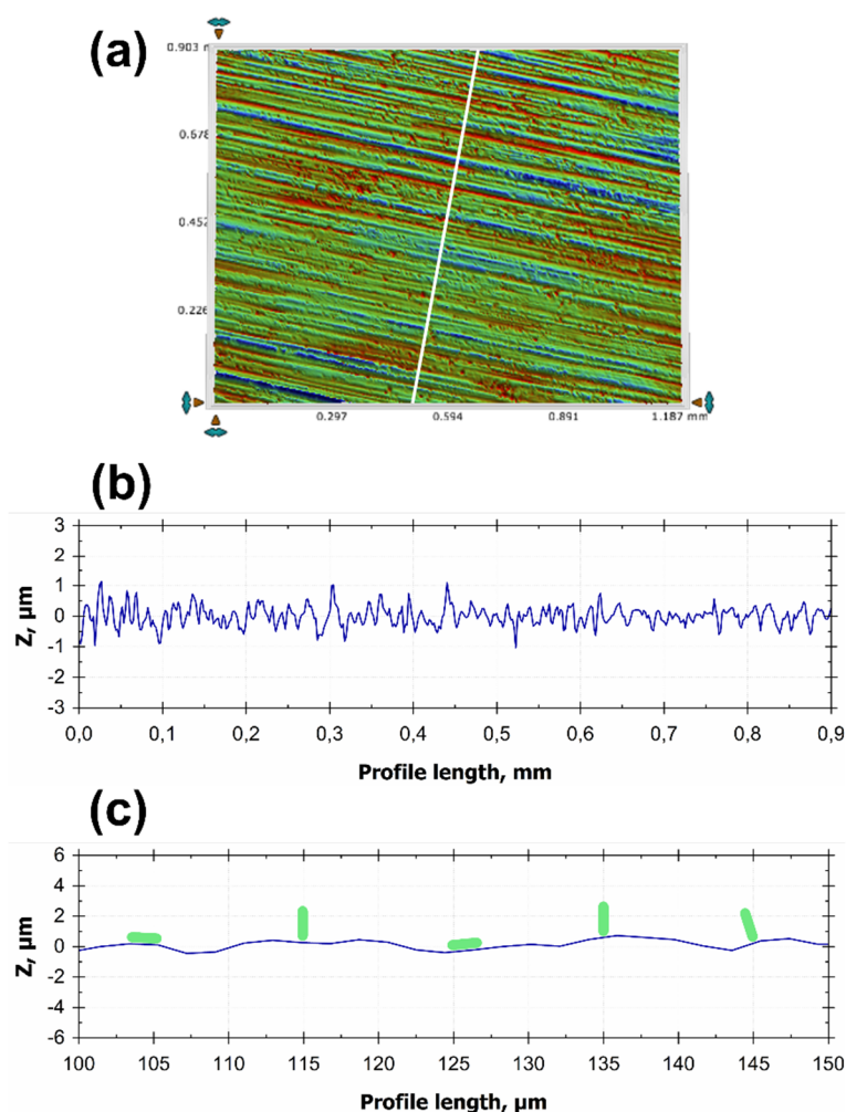
Figure 3.14. (a) Representation of the topography of the flat-like LSR surface of Shore A stiffness 59 at 1.2 \times 0.9 \text{ mm}^2 area. The white line indicates the position of the analyzed profile (b) Surface profile of the flat-like LSR taken in the perpendicular orientation to the grooves (profile length 900 \mu\text{m} ). The z-axis is stretched by a factor of 36. (c) A part of the same profile represented at a real scale, to visualize the surface roughness (profile length 50 \mu\text{m} ). Light-green pellets represent to-scale E. coli cells placed in arbitrary positions.
