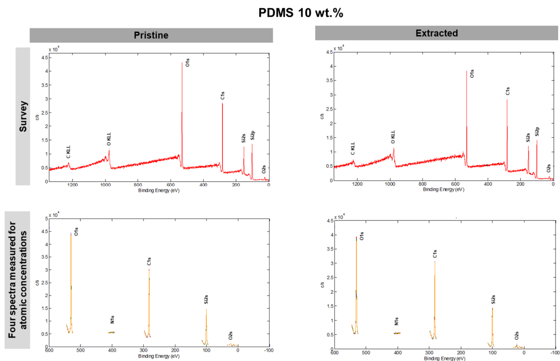
Figure S5. XPS survey spectra and four element spectra of O1s, N1s, C1s, Si2p, O2s regions for pristine and extracted PDMS with 10 wt.% of the cross-linker
