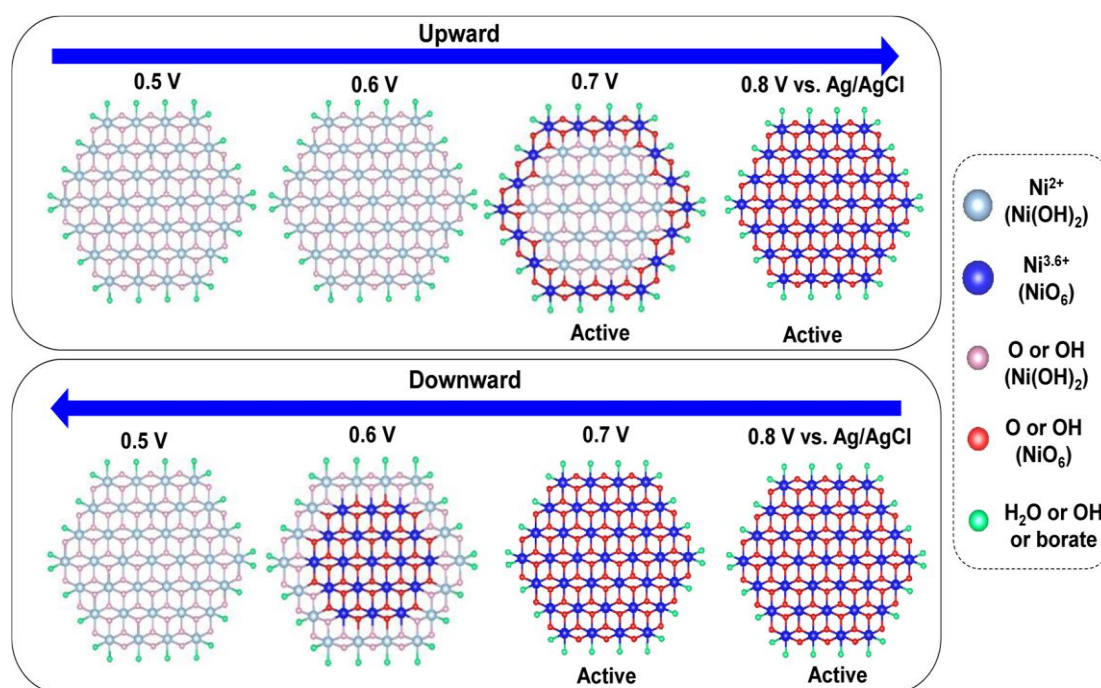
Figure 7: Schematic model for nickel nanocluster in the Ni-Bi electrocatalyst during OER catalysis in KBi aqueous solution with the electrode potential swept upward and downward (reproduced from ref. 20 with the permission from the American Chemical Society, Copyright 2012).
