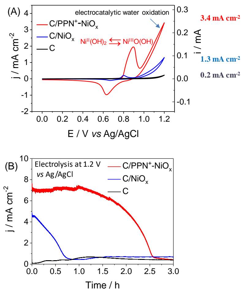
Figure 1: (A) Cyclic voltammograms (CVs) of C/PPN + -NiO x (red) ( \Gamma_{N^+} = 1.1 \times 10^{-7} \text{ mol cm}^{-2} , \Gamma_{Ni} = 3.3 \times 10^{-8} \text{ mol cm}^{-2} ) and C/NiO x (blue) ( \Gamma_{Ni} = 1.2 \times 10^{-8} \text{ mol cm}^{-2} ) electrodes (in black, the electroactivity of a naked C electrode of 3 mm diameter) in an aqueous 0.1 M borate buffer solution (pH 9.2), scan rate 50 \text{ mV s}^{-1} . (B) Chronoamperograms recorded at C/PPN + -NiO x (red) and C/NiO x (blue) (C electrode of 3 mm diameter) in a stirred 0.1 M aqueous borate buffer solution (pH 9.2), at constant potential of +1.2 V vs Ag/AgCl (adapted from ref. 11 with permission from the Royal Society of Chemistry, Copyright 2018)
