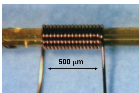
Figure 4.1: Hand winded solenoidal coil measuring sub nL samples [119].
