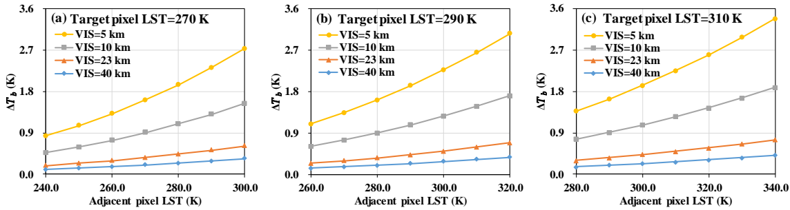
Fig. 2-15. Adjacency effect [defined as per Eq. 2-19] as a function of adjacent pixel temperature. Aerosol type, wavelength, image spatial resolution, and LSE were RURAL, 10 \mu\text{m} , 30 m, and 0.98, respectively. Target pixel temperature (TAT_LST) was (a) 270 K, (b) 290 K, and (c) 310 K. Adjacent pixel temperature varied from TAT_LST - 30 K to TAT_LST + 30 K, with a step of 10 K.
