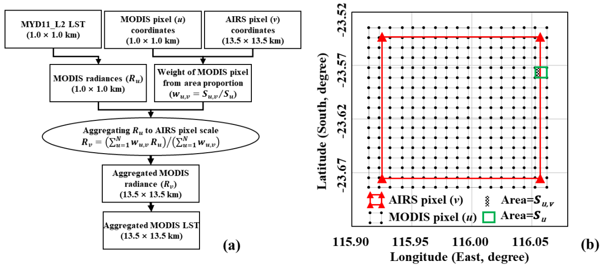
Fig. 4-16. (a) Flow diagram of the MODIS LST aggregating process, where N is the total number of MODIS pixels u inside or overlapped by one AIRS pixel v . (b) Illustration of the relationship between AIRS and MODIS pixel coordinates, where S_{u,v} is the area of overlap between pixels u and v and S_u is the total area of pixel u .
