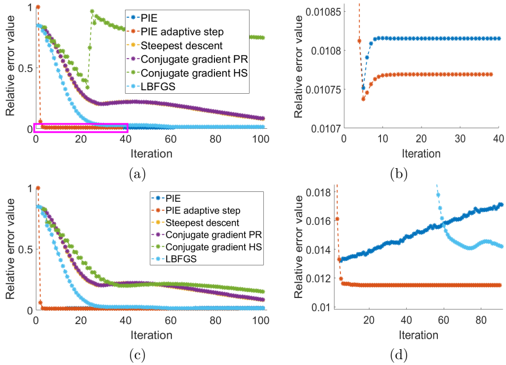
Figure 2.17: The relative error plotted as a function of the number of iterations. (a) The results for the noiseless case S_1 . (b) A zoom on the magenta zone to highlight the differences between PIE and PIE with the adaptive step methods. (c) Evaluation on a reconstruction from the data corrupted by Poisson-Gaussian noise S_2 . (d) A zoom on the PIE and PIE with the adaptive step methods.
