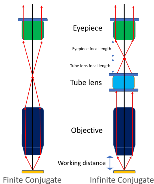
Figure 1.3: Finite conjugate and an infinite conjugate objectives. Reprinted from theonlinethoughts.com.
