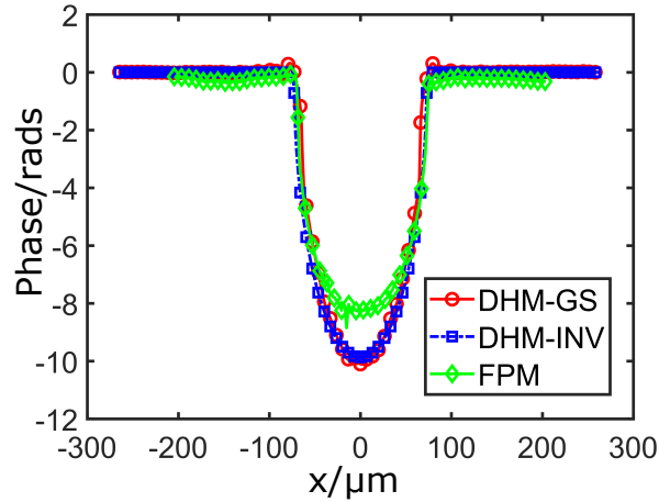
Figure 4.6: Phase curves recovered by LI-DHM and FPM. Curve with red circles is obtained by LI-DHM G-S algorithm. Curve with blue squares is phase distribution simulated according to Eqs 4.1, with diameter estimated from Fig. 4.1 and maximum phase shift provided by LI-DHM inverse problem approach. Curve with green diamonds represents phase retrieved from FPM G-S algorithm.
