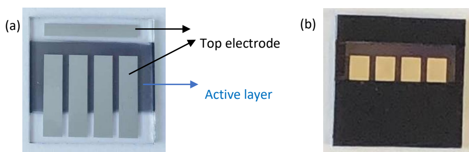
Figure 2.7 (a) The OPV sample and (b) shadow mask used for JV characteristics.
