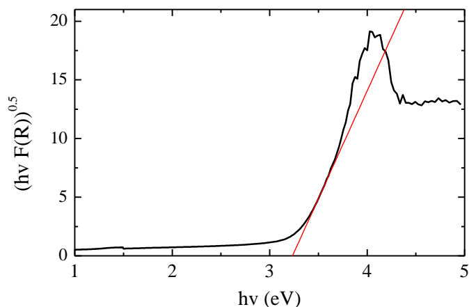
Figure 2.10. Tauc plot for 5 nm anatase \text{TiO}_2 particles for an indirect allowed transition ( n=2 ).
