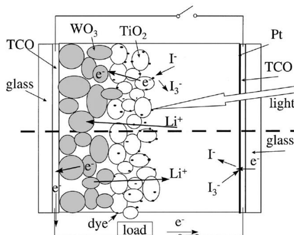
Figure 1.9. Schematic representation of the “photovoltaically self-charging battery” proposed by Orel et al. [29].
