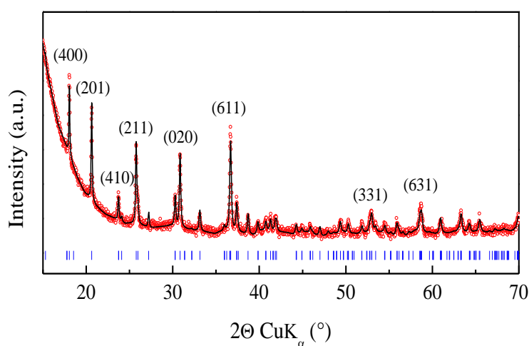
Figure 3.76. Full pattern matching refinement of the chemically obtained \text{FePO}_4 powder.
