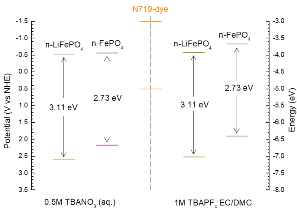
Figure 3.79. Energy diagram of the band edge positions of \text{LiFePO}_4 and \text{FePO}_4 measured in 0.5 mol/L \text{TBANO}_3 aqueous electrolyte and recalculated for pH = 14 (on the left), and in non-aqueous aprotic 1 mol/L \text{TBAPF}_6 EC/DMC-based electrolyte (on the right). The information on the HOMO and LUMO levels of N719-dye is provided for comparison [218].
