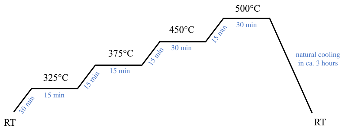
Figure 2.3. Schematic representation of the 4-step heat-treatment procedure to remove ethyl cellulose and terpineol from the screen-printed \text{TiO}_2 electrodes.
