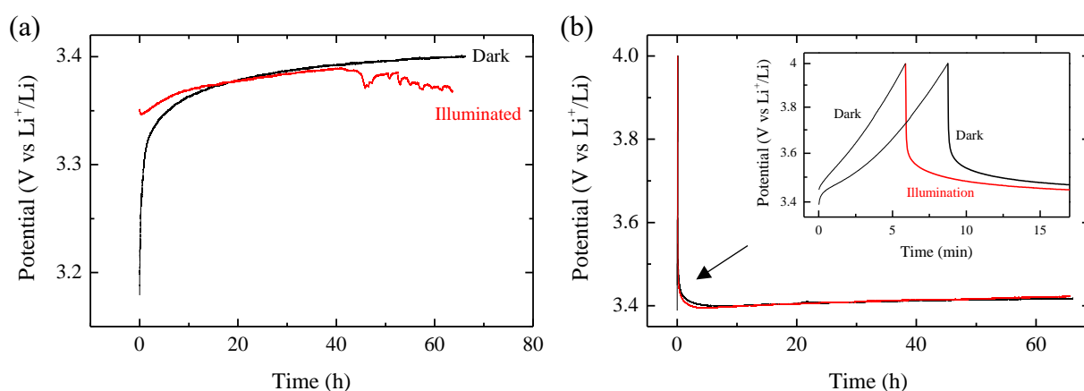
Figure 3.73. Evolution of open circuit potential in dark or under illumination under A.M. 1.5G conditions (a) from \text{LiFePO}_4 (b) from " \text{FePO}_4 " obtained after galvanostatic charge to 4.0 V vs \text{Li}^+/\text{Li} at 10 \mu\text{A}/\text{cm}^2 .
