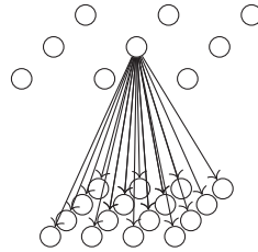
Figure 3.10.: Local illustrations of the correlations within the quadtree SBN model: all the sons of a father vertice.
