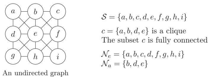
Figure 1.1.: Examples and notations of graph theory I.
