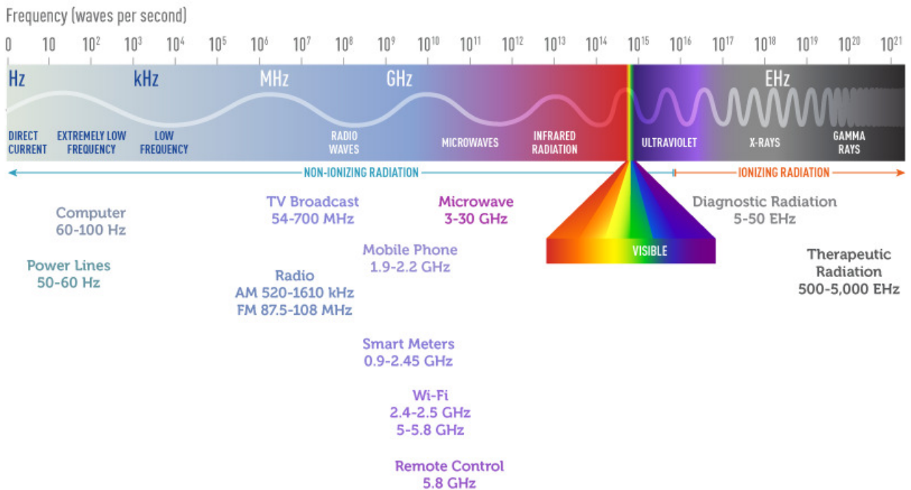
Figure 1.1: The electromagnetic spectrum. Source: NCI [1]
