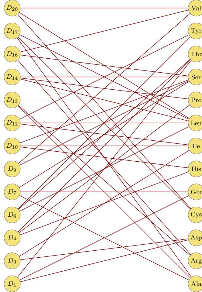
Figure 4.3: The bipartite graph \mathcal{G} = (V, E) where V is composed of the 13 equivalence classes in D = \{D_1, D_3, D_4, D_6, D_7, D_9, D_{10}, D_{12}, D_{13}, D_{14}, D_{16}, D_{17}, D_{20}\} and the 13 amino acids in A = \{\text{Val, Tyr, Thr, Ser, Pro, Leu, Ile, His, Glu, Cys, Asp, Arg, Ala}\} , and E is the set of all pairs (D_i, aa) such that there is a codon in D_i that encodes the amino acid aa .
