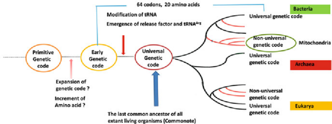
Figure 1.7: A schematic presentation of the microbiological evolution introduced in [74]. The evolution line marks the important milestones of the evolution. Starting with a primitive code which first evolved to the early genetic code and then to the LUCA (last common ancestor code). After LUCA, the branches of evolution divide into the forms of life we have today. (Picture taken from [74])
