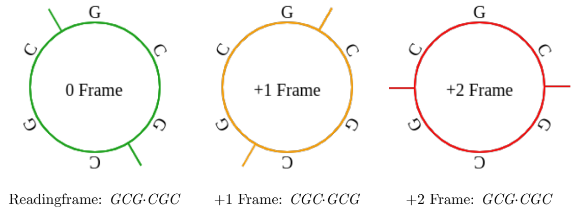
Figure 1.10: An illustration of the three reading-frames of the sequence GCG \cdot CGC . All three frames are decomposed into the same words.
