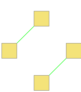
Figure 3.14: \varphi(\mathcal{C}_2(\mathcal{X}_j)) if |A||B||C| = 00X with X \in \{0, 2\} . The green edges represent the value of X
