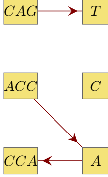
Figure 1.14: \mathcal{C}_1(\mathcal{X}) of the representing graph \mathcal{G}(\mathcal{X}) of the code \mathcal{X} = \{ACCA, CAGT\}
