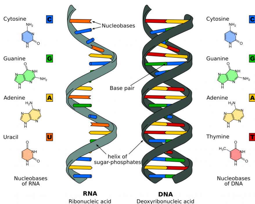
Figure 1.2: This figure demonstrates the difference of the single stranded RNA and DNA double helix. On the margins of the picture, the structures of the nucleobases are presented. (Picture taken from https://teachmephysiology.com/biochemistry/protein-synthesis/dna-transcription )
