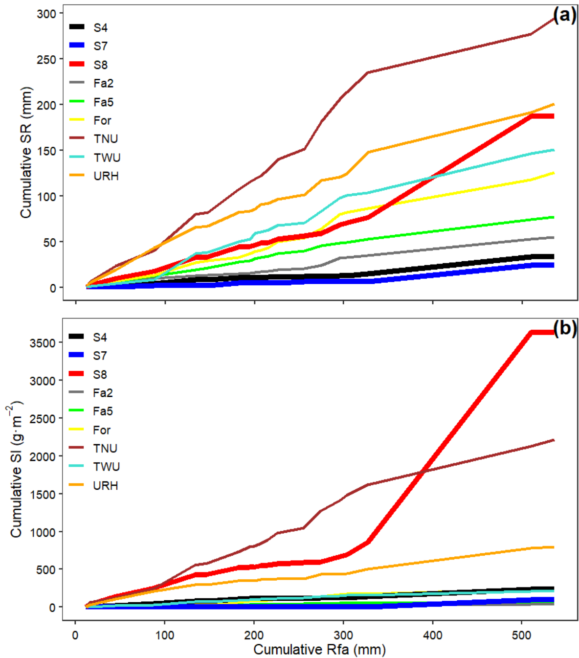
Figure 6.4: (a) Cumulative surface runoff (SR; mm) versus cumulative rainfall (Rfa, mm), and (b) cumulative soil loss (Sl; \text{g}\cdot\text{m}^{-2} ) versus cumulative Rfa, in the catchment (S4), the micro-catchments (S7 and S8), and the microplots (Fa2, Fa5, For, TNU, TWU, and URH), measured from 8 July to 22 September 2014, in Houay Pano catchment, northern Lao PDR. Fa2: fallow of 1 – 3 years; Fa5: fallow of 4 – 15 years; For: forest; TNU: teak without understory; TWU: teak with understory; URH: upland rice.
