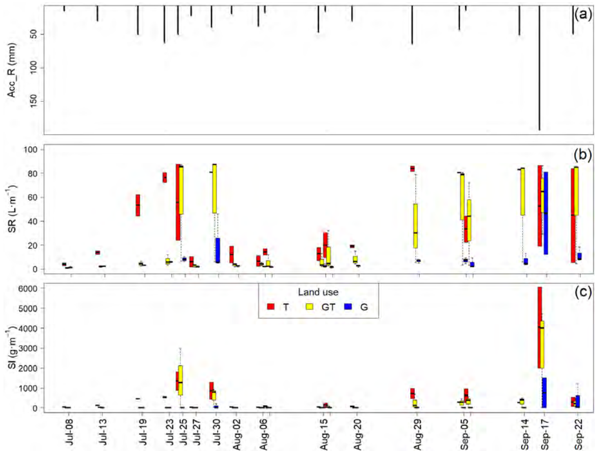
Supporting Figure 5-6. Gerlach traps: (a) accumulated rainfall between two samplings (Acc_R, mm); boxplot of (b) surface runoff (SR, L \cdot m^{-1} ), and (c) soil loss (Sl, g \cdot m^{-1} ) for three land uses from 8 July to 22 September 2014, in Houay Pano catchment, northern Lao PDR. T: teak with no understory; GT: grass with teaks; G: grass. Each rainfall bar represents the cumulative rainfall over two to twenty-three rainfall events, or after every major event (event whose rainfall triggered the sampling). Each boxplot contains the extreme of the lower whisker (dashed line), the lower hinge (thin line), the median (bold line), the upper hinge (thin line), and the extreme of the upper whisker (dashed line). The whiskers extend to the most extreme data point, which is no more than 1.5 times the interquartile range from the box.
