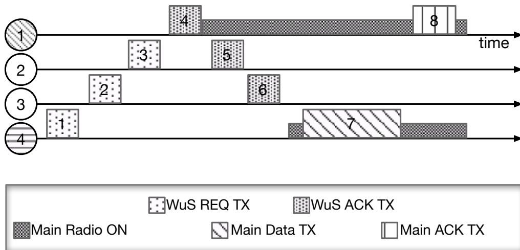
Figure 3.3: WuSACK protocol timeline
