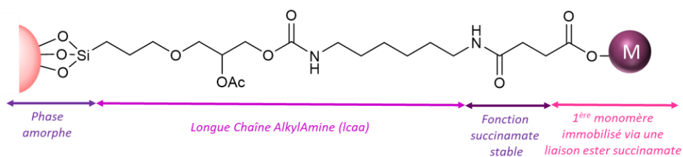
Figure I. 19: Structure du support solide lcaa standard.
