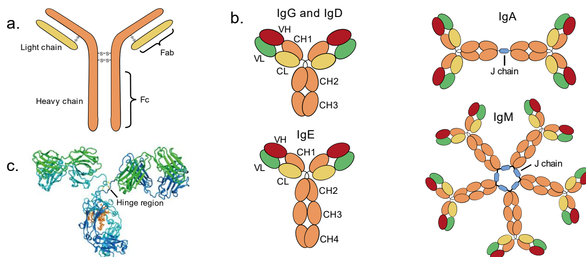
Figure 28. Schematic illustration of (a) antibody structure, (b) different antibody isotypes and (c) ribbon representation of intact immunoglobulin. (a) Antibody sketch to demonstrate the interactions of heavy chains and light chains, as well as disulfide bonds in intact immunoglobulin molecule. Heavy chains in orange and light chains in yellow connected by disulfide bonds (structure corresponding to IgG1, displaying two disulfides at the hinge area); (b) Different immunoglobulin isotypes comprising monomeric IgG and IgD consisting of four heavy chain and two light chain immunoglobulin domains, monomeric IgE consisting of five heavy chain and two light chain immunoglobulin domains, dimeric IgA having the same constant and variable domain structure as IgG and IgD, pentameric IgM having the same constant and variable domain composition as IgE. Antibody moieties in IgA and IgM are connected via the joining (J) chain; (c) Ribbon representation of intact immunoglobulin (mouse IgG2A isotype), structure obtained from Protein Data Bank (PDB) 207
