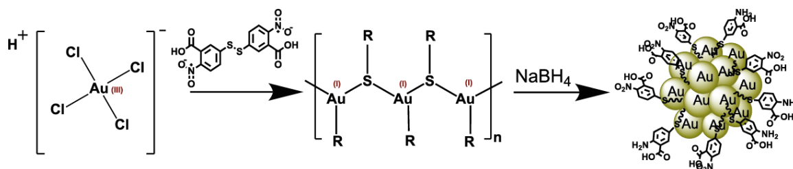
Figure 15. Synthesis strategy for generating TAB-/ TNB-protected AuNPs by reducing \text{HAuCl}_4 in the presence of DTNB with \text{NaBH}_4 .
