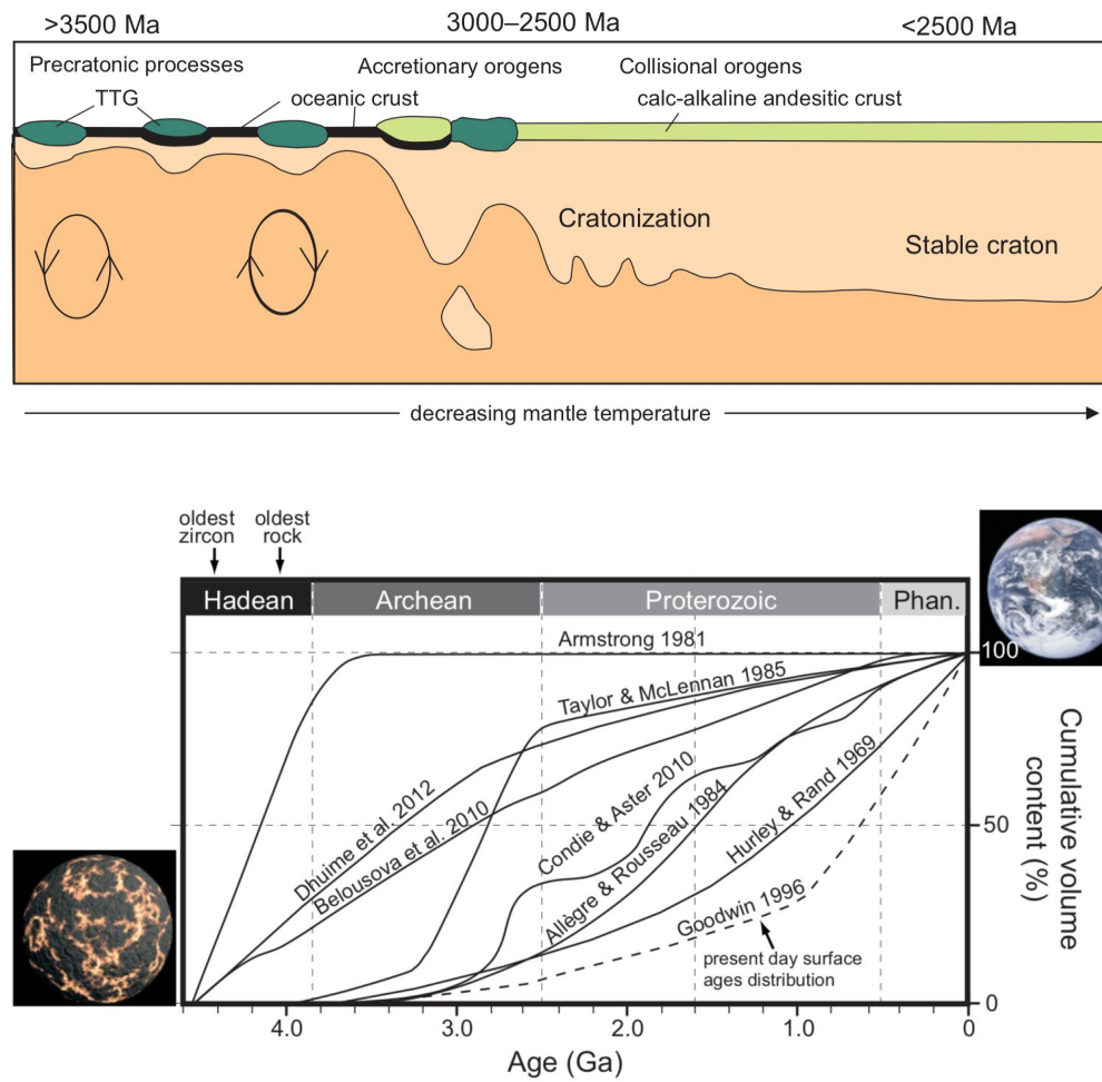
Figure 1.6: (Top panel) Temporal evolution of the lithosphere associated with the thermal evolution of the mantle from early Earth (adapted from S. Foley, 2012, personal commun.) involving a bimodal association of TTG (tonalites, trondhjemites, and granodiorites) and greenstone evolving through development of accretionary and collisional orogenic processes into a regime producing continental crust of andesitic composition by at least 3.0 Ga. (Bottom panel) Crustal growth models of Hurley and Rand (1969), Armstrong (1981), Allègre and Rousseau (1984), Taylor and McLennan (1985), Condie and Aster (2010), and Dhuime et al. (2012) compared to age distributions of presently preserved crust Goodwin (1996). Figure and caption from Cawood et al. 2013.
