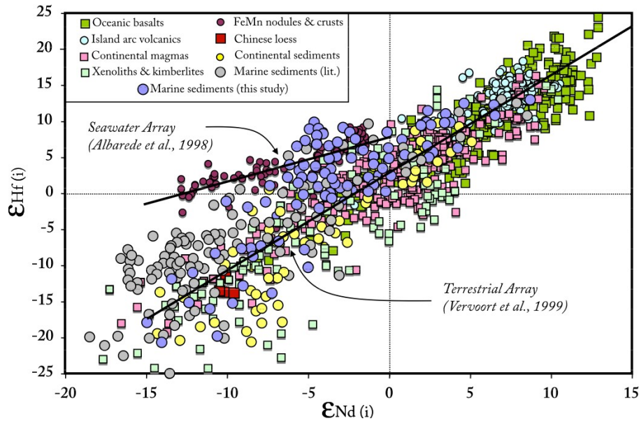
Figure 1.9: Initial \epsilon_{\text{Nd}} vs. \epsilon_{\text{Hf}} for representative crust and mantle compositions. To a first order, all compositions form a strong positive correlation called the Terrestrial Array. The most obvious deviations from this are Fe-Mn crusts/nodules, which define a seawater array. Reference Terrestrial Array ( \epsilon_{\text{Hf}} = 1.36 \times \epsilon_{\text{Nd}} + 2.95 ) and seawater array ( \epsilon_{\text{Hf}} = 0.55 \times \epsilon_{\text{Nd}} + 7.1 ) after Vervoort et al. (1999) and Albarède et al. (1998), respectively. Figure and caption from Vervoort et al. 2011.
