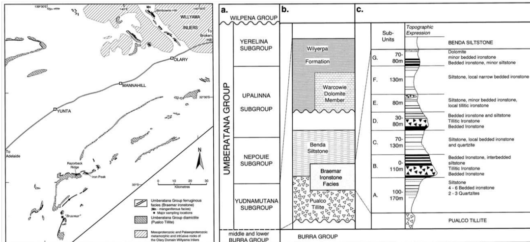
Figure 4.2 (Left panel) Geographical location of outcrops and sampling sites of the Braemar Formation in South-central Australia. (Right panel) Stratigraphic column of the Neoproterozoic Braemar Ironstones. The column highlights the paucity in the IF formation as well as its close association with glacially derived sediments. From Lottermoser and Ashley (2000).
