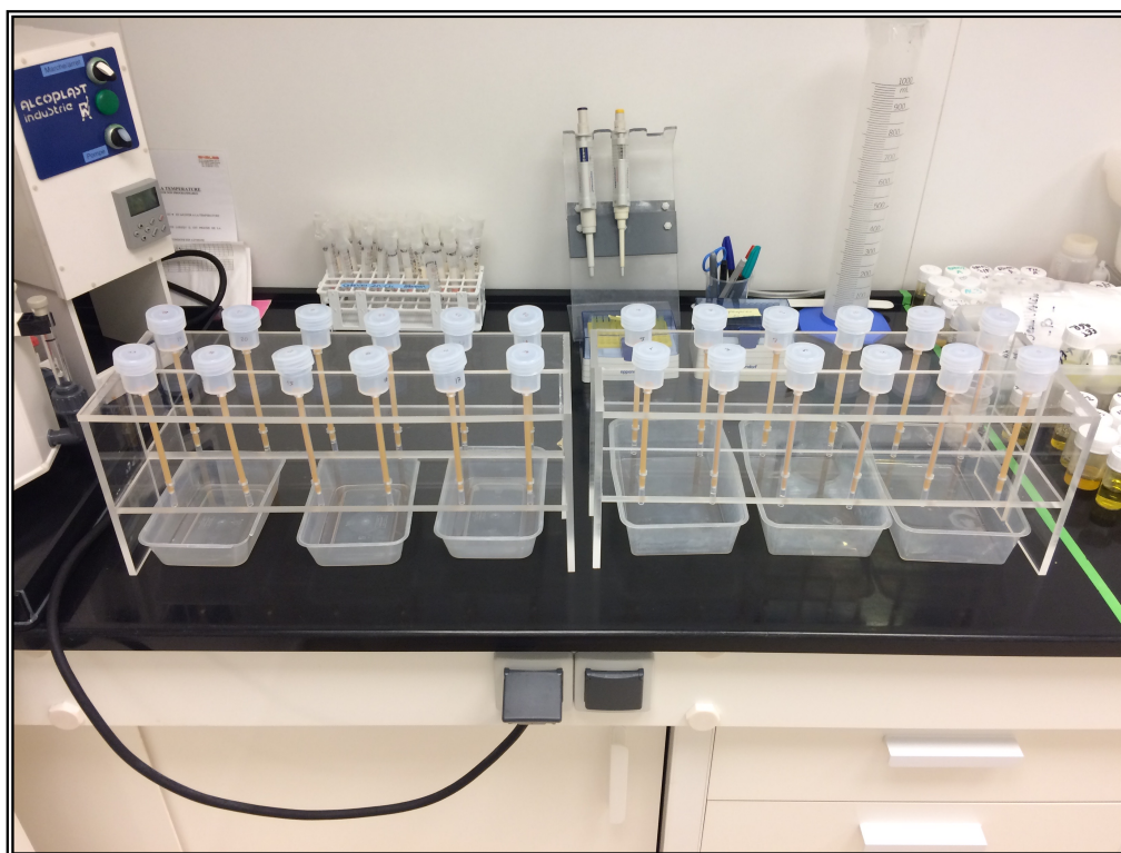
Figure 2.11: Long Teflon columns prepared and conditioned in 2.5 N HCl ready for use as described in the protocol above.
