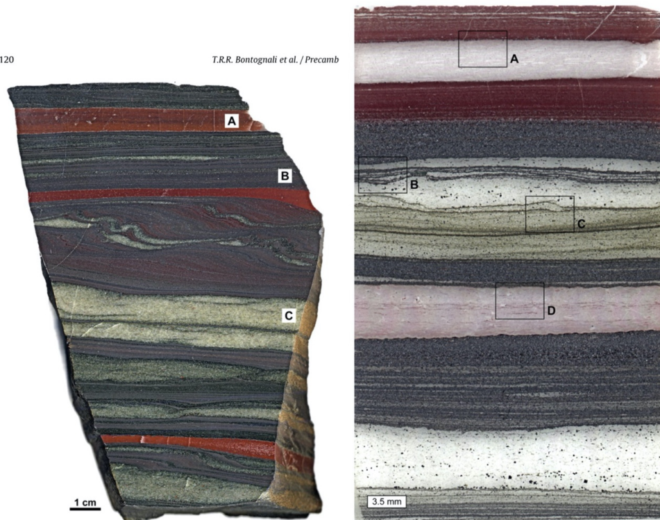
Figure 1.17: (Left panel) Photograph of a polished slab of Moodies BIF. (A) Chert concretion. (B) Sub- mm scale laminations of iron-bearing minerals (mainly magnetite and hematite). (C) Siliciclastic bed. Chert concretions variably show mm to sub mm-scale internal laminations due to the variable amount of incorporated iron minerals. Iron-rich laminations are due to both the fine interlamination with siliciclastic material and the variable amount of surrounding chert. (Right panel) Large-scale photograph representative of a Moodies BIF polished sample. (A) Contact between two chert beds. The color of the chert varies from dark red to almost transparent depending on the concentration of microscopic iron minerals (primarily hematite). (B) Iron-rich microbands finely interlaminated with siliciclastic grains (mainly fine quartz sand). (C) Siliciclastic bed showing laminations comprised of sand draped by iron-bearing minerals. (D) Chert bed including discontinuous laminae comprised of iron minerals. Figure and caption from Bontognali et al. 2013.
