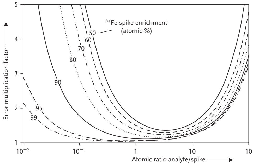
Figure 2.12: Error multiplication factors for isotope dilution mass spectrometry determination an element (example: iron) as a function of the analyte/spike atomic ratio for different spike enrichments of ^{57}\text{Fe} . From Isotopic Analysis (2012), Chapter 8.2.3, by Vanhaecke and Degryse.
