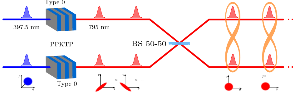
Figure 8.2 – Experimental setup for the production of entangled states. Two sources of pulsed squeezed states allow to produce quantum correlated pulses by mixing two squeezed pulses on a 50-50 BS. Those correlated pulses can be used as nodes for a quantum reservoir computing architecture.
