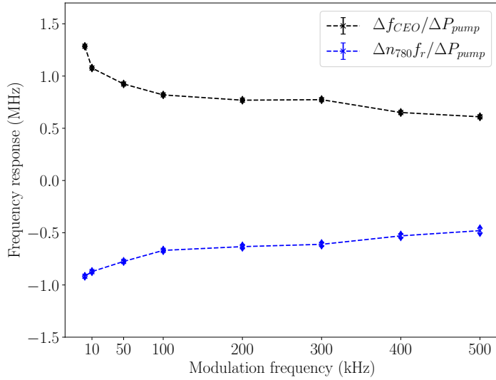
Figure 5.5 – Frequency response of the CEO frequency \Delta f_{CEO} and the repetition rate \Delta n_{780} f_r as a function of the modulation frequency. The fluctuations are less important at high frequencies due to the filtering of the cavity or due to thermal effects.
