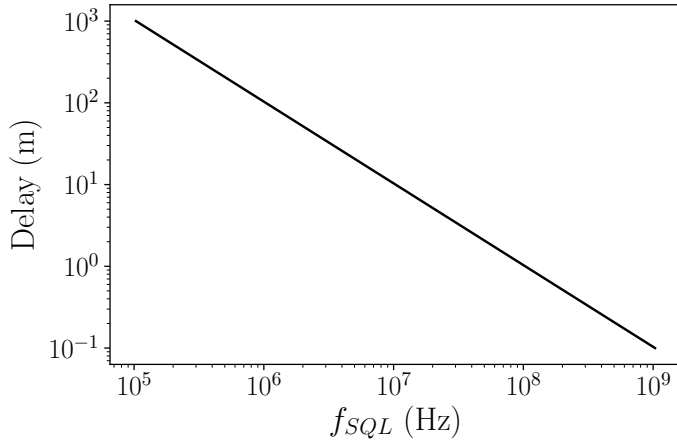
Figure 3.7 – Delay allowing to reach the best sensitivity. In order to achieve the best sensitivity given by equation (3.72) at the frequency f_{SQL} different delays must be employed. The delay is given by d = \tau \times v where v = c/1.45 is the speed of light in a silica optical fiber.
