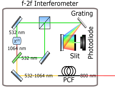
Figure 4.2 – Drawing of the f-2f interferometer. The initial spectrum is expanded thanks to a photonic crystal fibre to have a span of an octave. The signal at 532 nm is mixed with the one at 1064 nm but frequency doubled to measure the CEO of the laser.
