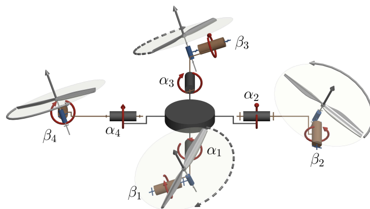
Figure 3.15 – Conceptual 3D kinematic representation of a generic quadrotor with propellers tilting/tilted in \mathbb{S}^2 , i.e., about both the radial and tangential axes.
