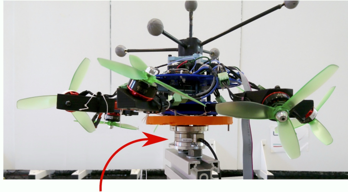
Force-Torque Sensor
