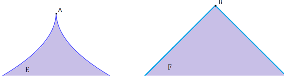
FIGURE 1. The point A belongs to \partial^-E but A \notin \partial_e E . The point B belongs to \partial_e F but B \notin \partial^* F .
