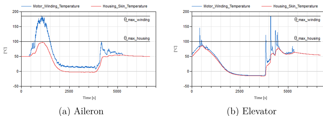
Figure 7.21: Thermal profile of EMAs designed with the thermal straps.
