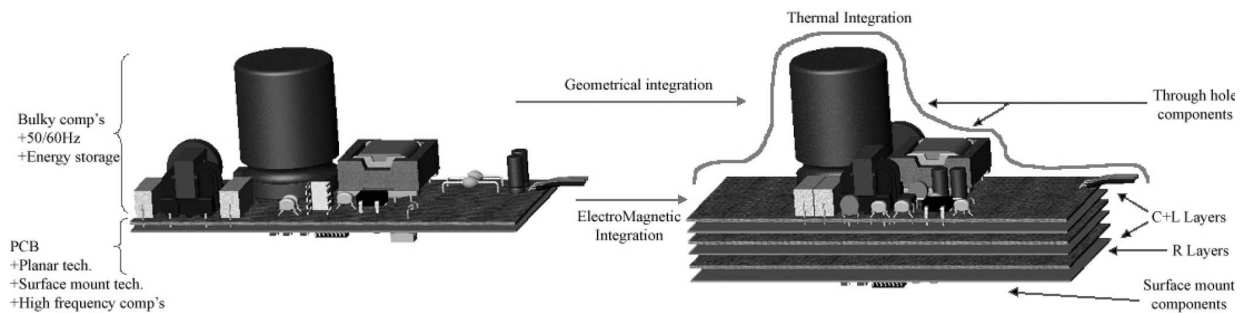
Figure 2.11: Conceptual integration process in switch mode converters from (left) discrete component design to (right) more integrated design [58].
