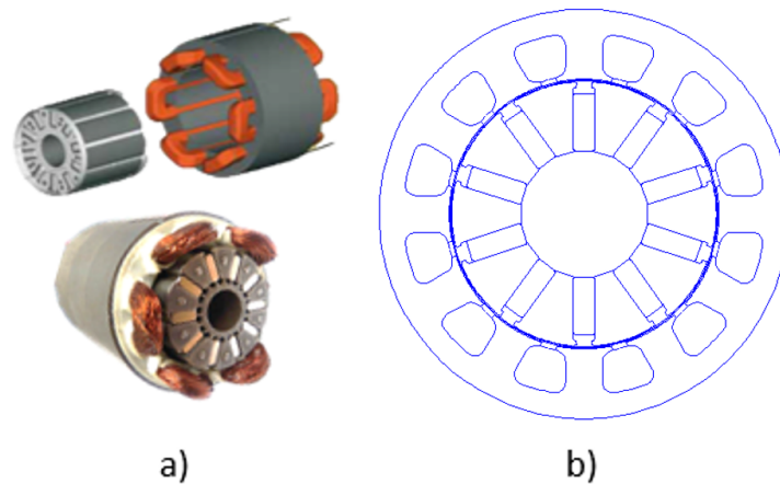
Figure A.1: a) Parvex NX 310 servomotor and b) its representative finite elements model.
