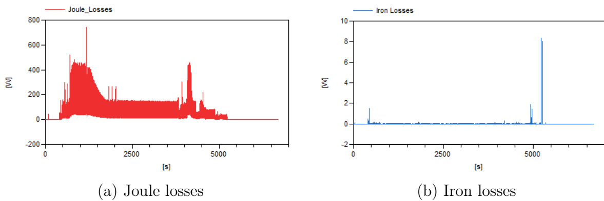
Figure D.4: Motor Losses (Aileron - Case study 1).
