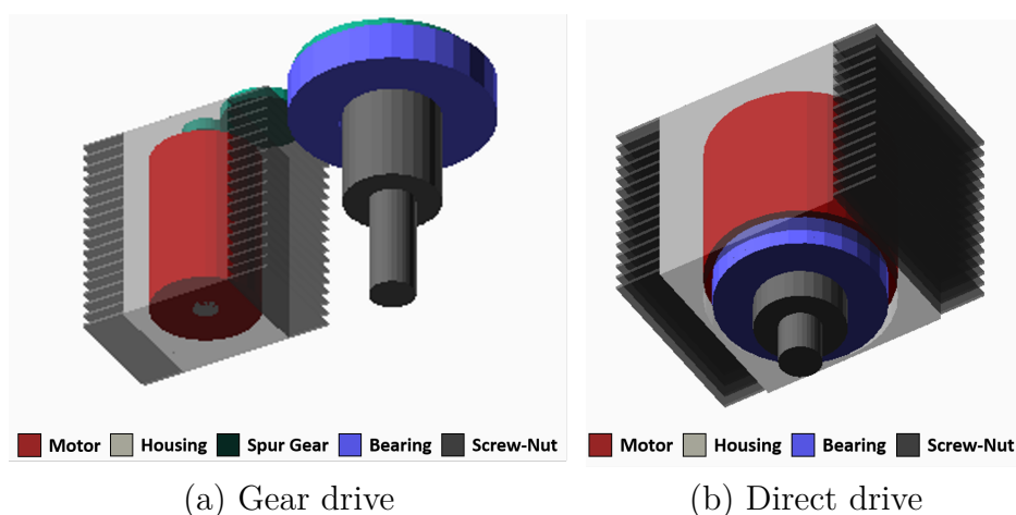
Figure 4.3: Considered EMA architectures for the case study.
