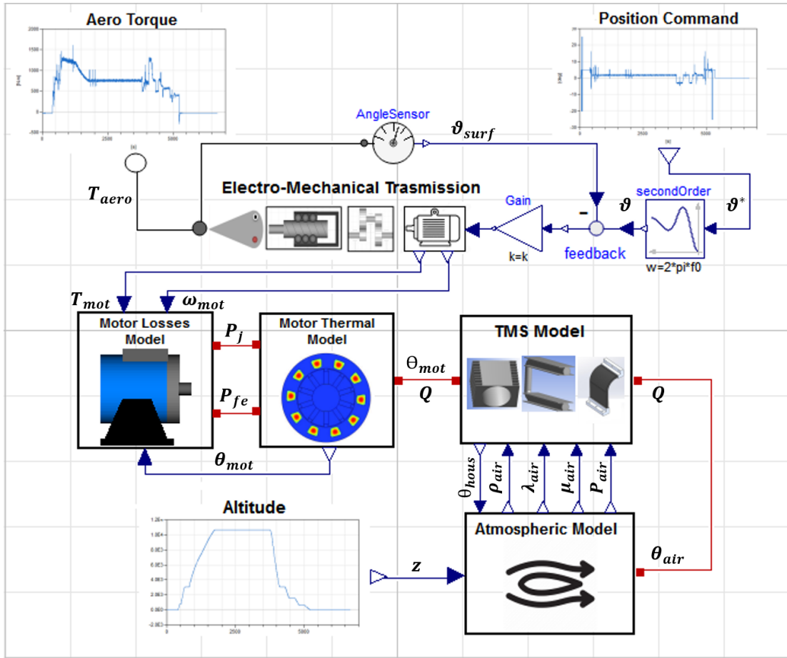
Figure 7.3: Actuator dynamic model architecture and interfaces.
