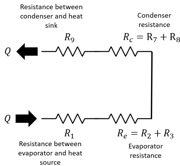
Figure 5.8: Simplified Heat Pipe Thermal Resistance Network.
