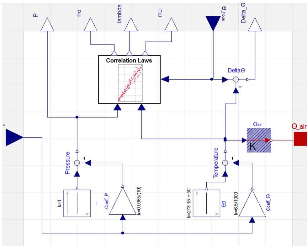
Figure 7.8: Atmospheric Model.
