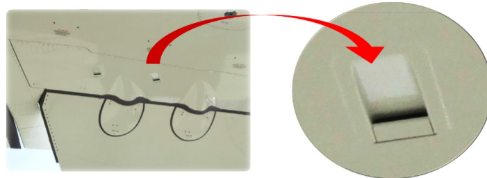
Figure 2.14: Underwing scoops for actuator cooling (EHA of the Airbus A350 aileron) [8].
