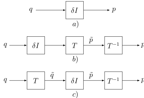
FIGURE 3.4: Equivalent representation of \delta I_{n_q}
