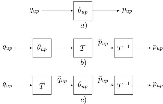
FIGURE A.3: Equivalent representation of \theta_{up}
