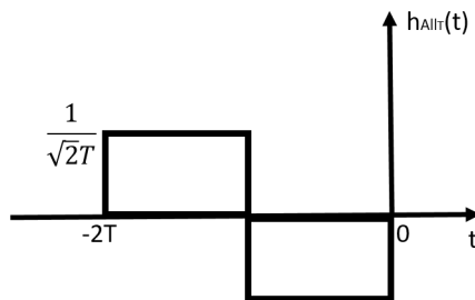
FIGURE 5.5: Impulse response
