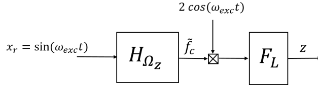
FIGURE 4.2: Extraction of the in-phase component
