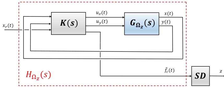
FIGURE 4.1: Closed-loop MIMO direct control
