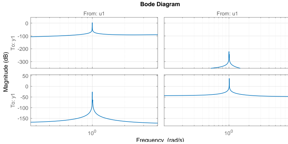
FIGURE 2.12: Identified model with cross-couplings
