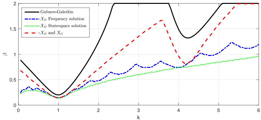
FIGURE 3.11: Stability domain of Mathieu-Hill equation with b = 0
