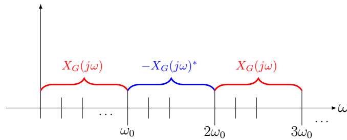
FIGURE 3.10: Construction of X_G(j\omega)
