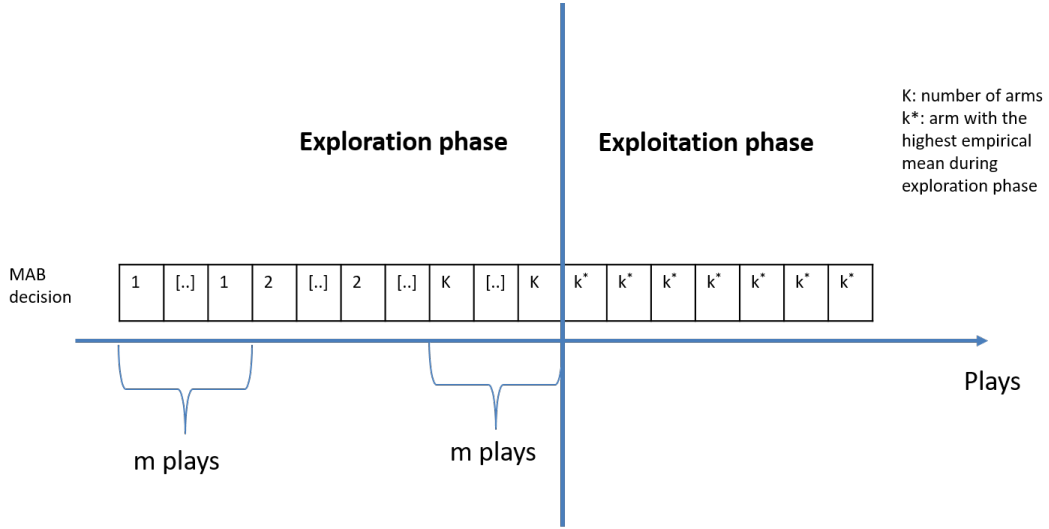
FIGURE 2.7: Explore-then-Exploit
