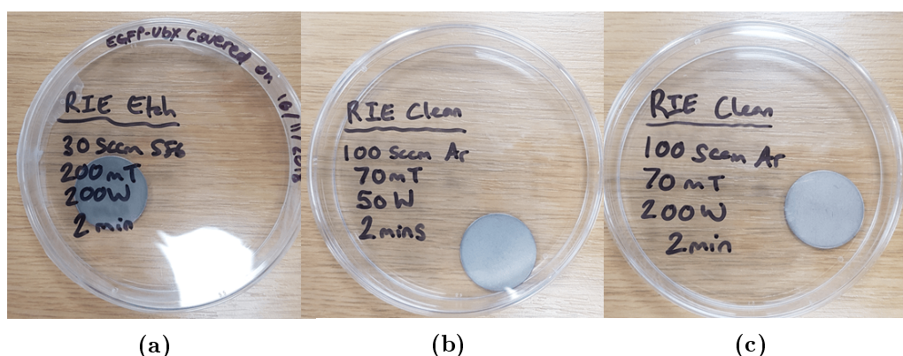
Fig. 5.13: Titanium discs cleaned for 15 minutes with IPA in a sonicator prior to do Plasma cleaning for 2 minutes with (a) SF_6 , with 30 sccm flow rate, p = 200 mT, P = 200 W; (b) Ar, with 100 sccm flow rate, p = 70 mT, P = 50 W; (c) Ar, with 100 sccm flow rate, p = 70 mT, P = 200 W.
