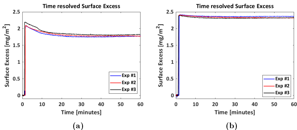
Fig. 6.5: Time-resolved surface excess of old proteins spread in 0.1 M NaCl using \text{H}_2\text{O} (a) and \text{D}_2\text{O} (b) as subphase.
