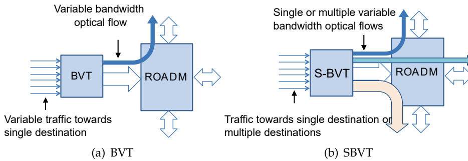
Figure 1.9: Illustration of BVT and S-BVT in FONs[44].
