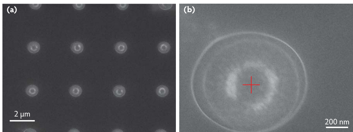
Figure 4.6 Alignment marker for e-beam lithography
