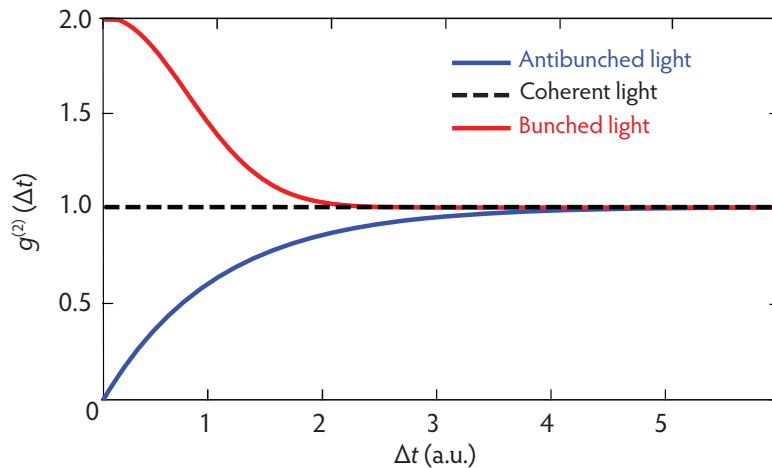
Figure 1.15 Antibunched, coherent, and thermal light
