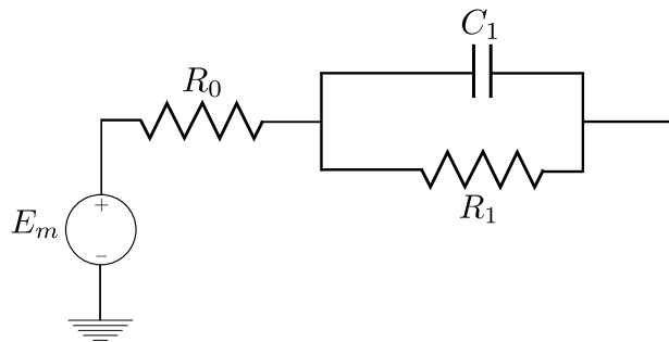
Figure III.4: Adapted Thevenin equivalent model of the Li-ion battery.
