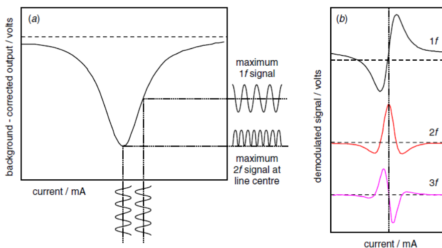
Figure A1.1.1: Generation of different harmonic signals in wavelength modulation spectroscopy. a) DC scan through a single gas line, b) Form of 1f , 2f and 3f harmonics as a function of position in the current scan. [1]
