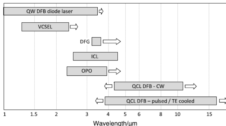
Figure 1.2.2. Wavelength coverages for various light emitters. Arrows show the direction of research activity in a developing field. The abbreviation indicate CW: continuous wave, QW DFB: quantum well distributed feedback, DFG: difference frequency generation, ICL: interband cascade laser, OPO: optical parametric oscillator, QCL: quantum cascade laser. [19]
