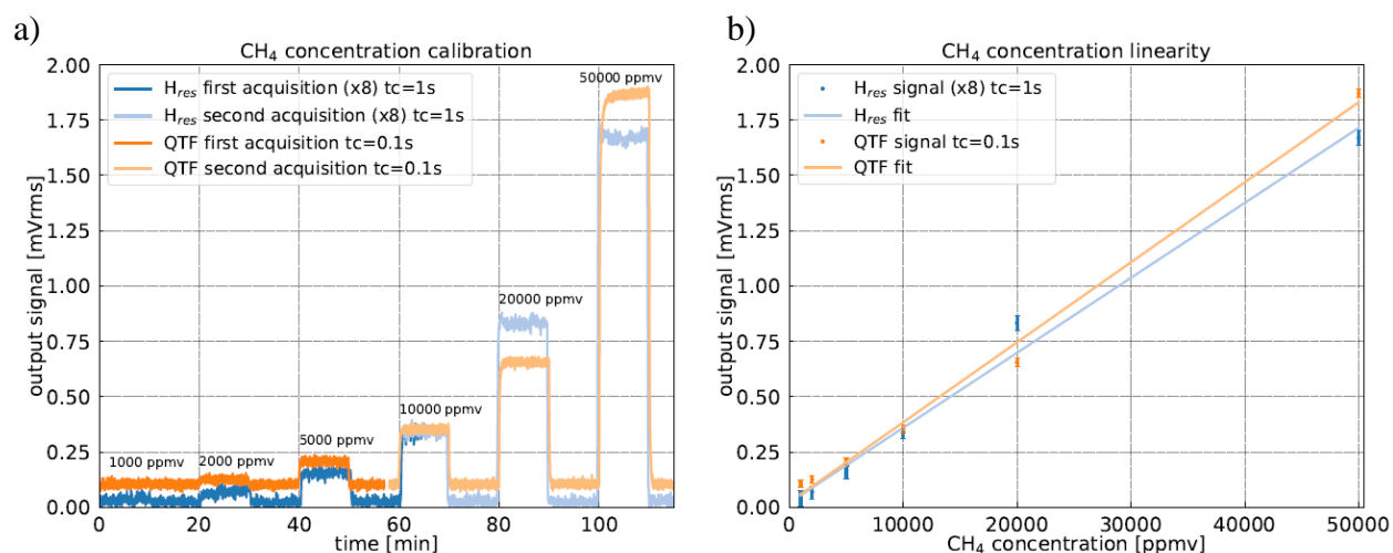
Figure 5.6.3: a) 1f QEPAS (orange) and H-resonator (blue) signal during continuous measurement with a gas step cycle. Concentration was ranging from 1000 ppmv to 50000ppmv. After injecting a known concentration of methane for 10 minutes, the cell is flushed with pure \text{N}_2 for 10 minutes. (b) Signal from QEPAS (orange) and H-resonator (blue) as a function of injected methane concentration with a linear fit of the response. The integration time is 0.1 s for QEPAS and 1 s for H-resonator.
