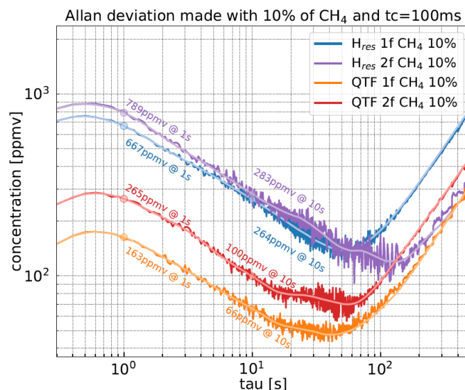
Figure 5.6.4: Allan-Werle deviation for QTF and H-resonator calculated from a 30 minutes acquisition for the 1f and 2f mode with 10% of CH 4 concentration and time constant of 100ms.
