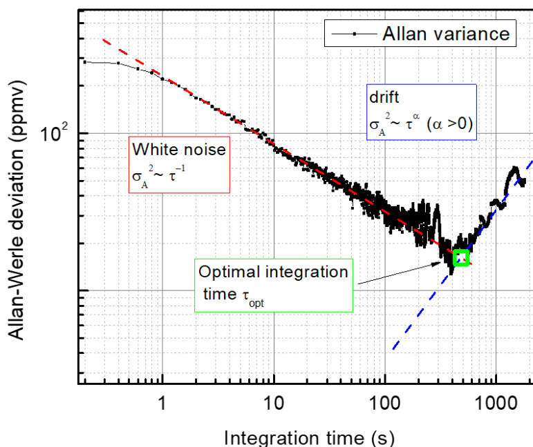
Figure 4.4.9. Allan – Werle deviation calculated for XRE.FP from 30 min acquisition for 1f detection with 1% of \text{CH}_4 . Time constant 200 ms, optical read-out mechanism. White noise is dominating when \sigma_A^2 \propto \tau^{-1} (red slope), drift dominated region occurs for \sigma_A^2 \propto \tau^\alpha (where \alpha > 0 , blue slope). Beyond the drift noise and white noise exist an optimal integration time \tau_{opt} .
