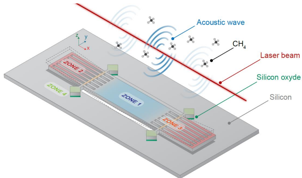
Figure 5.1.1: H-resonator design with the schematic representation of deflection under PA excitation. The laser beam is focused above the resonator's center and is aligned along the resonator's x-axis. The absorption of modulated light generates an acoustic wave all along the beam.
