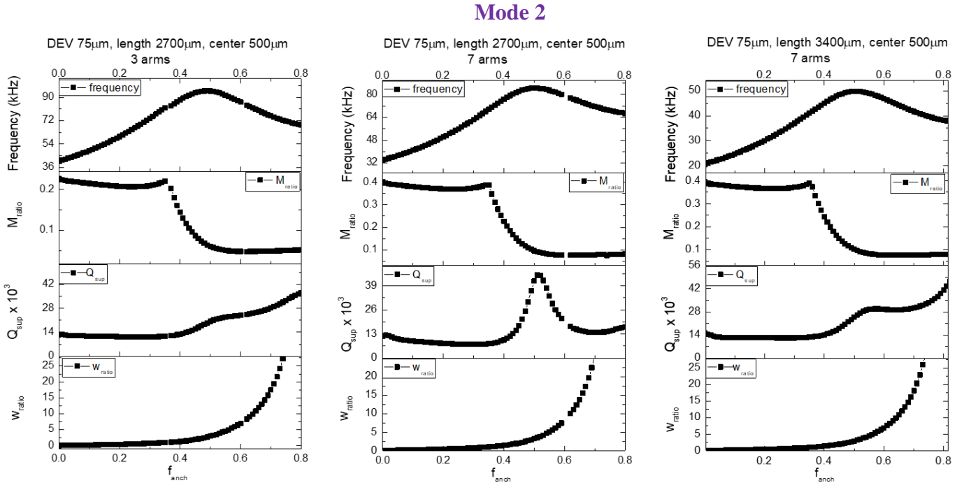
Figure 5.3.4. Results from the COMSOL simulation of chosen H-resonator as a function of anchor position expressed with factor f_{anch} . Parameters of H-resonator included above the graphs; where DEV informs about a device thickness, length is L_{tot} , center is center size, M_{ratio} is the mass ratio given by equation (5.2), Q_{sup} is a support quality factor, w_{ratio} is the ratio of displacement between extremity of zone 2 and center of zone 1 introduced in chapter 4.
