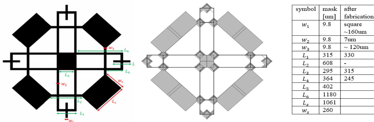
Figure 4.3.6: a) Geometry scheme of XRE.F presented on the photolithography mask and b) geometry scheme which represents XRE.F after fabrication. Figure presented on the right panel was created using COMSOL Multiphysics Software.
