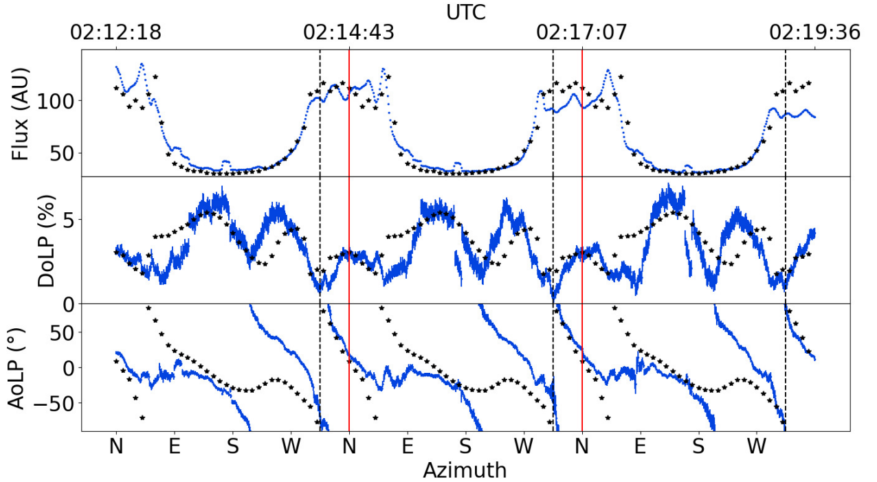
Fig. 12: 3 almucantar observations at 427.8 \pm 5 nm (Feb. 2019): observations (in blue) and predictions for the model that best fits the data (Black stars ★). The model is a linear combination of ground and sky (including albedo) for a 6% polarised sky emission in a direction defined by an azimuth of 50^\circ and 10^\circ elevation (see text for details). The dashed vertical black line indicates the direction of Skibotn. The picture of the sky at 557.7 nm is shown in Appendix A.
