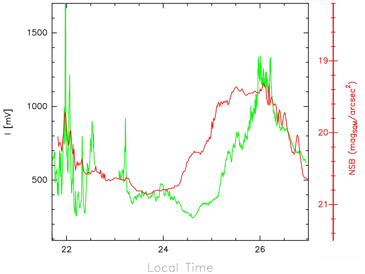
Fig. B.1. This figure compares the Ninox data (in red) to the green line polarimeter flux as in Figure 3 (green line).
