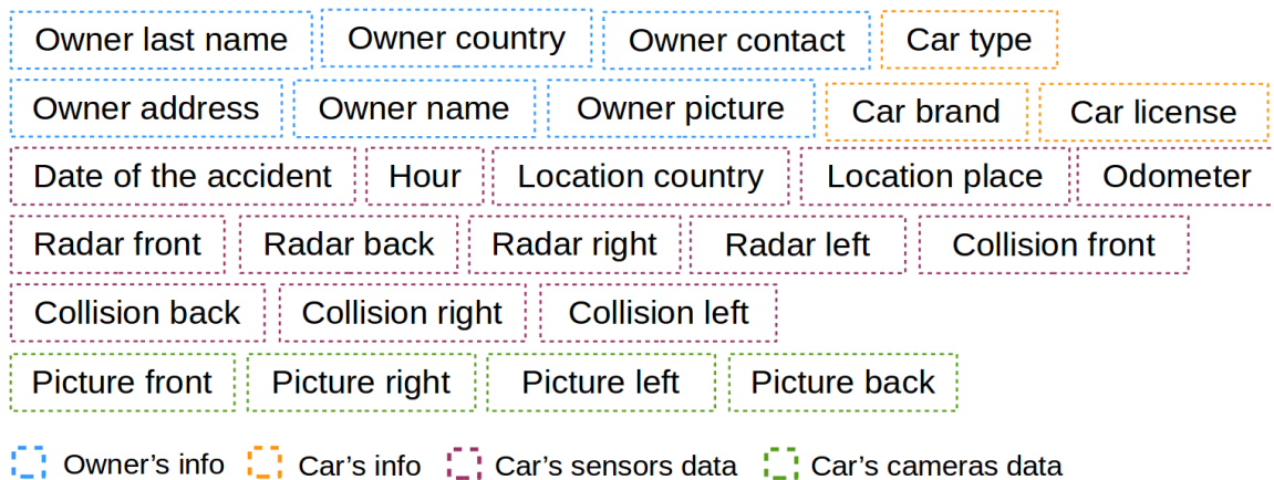
Figure 3.14: Example of the transaction payload that sent when an accident occurs
