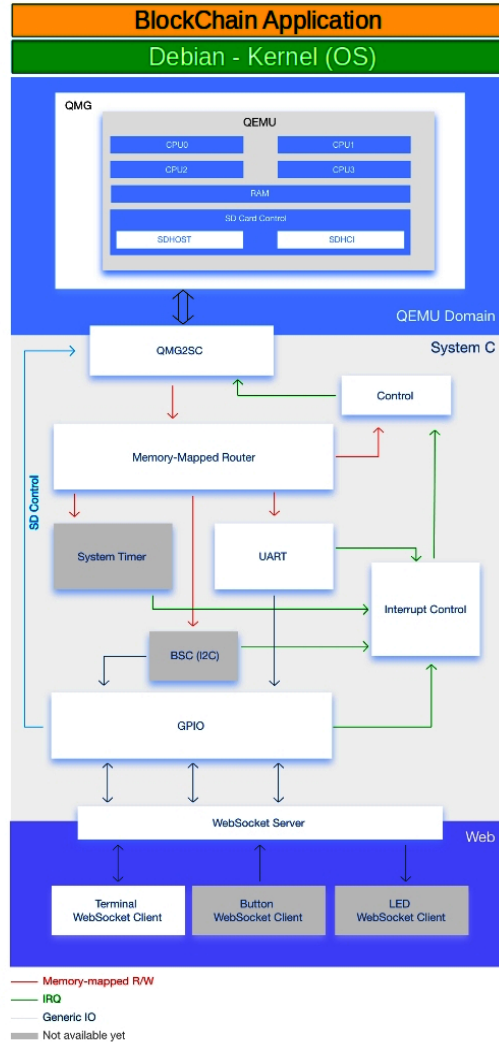
Figure 5.7: BCM2837 architecture modelled by Hivertive QEMU-SystemC platform. The figure is adopted from [17]
