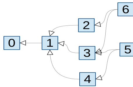
Figure 2.10: Example of a Directed Acyclic Graph
