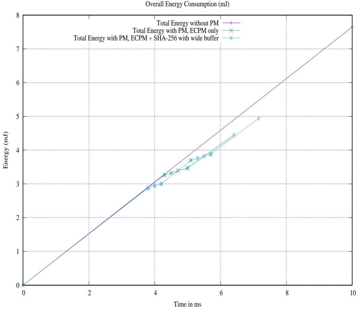
Figure 5.23: Overall Energy Consumption of EOS.IO API, retrieved by using PwClkARCH. PM in the titles of the curves means Power Management.
