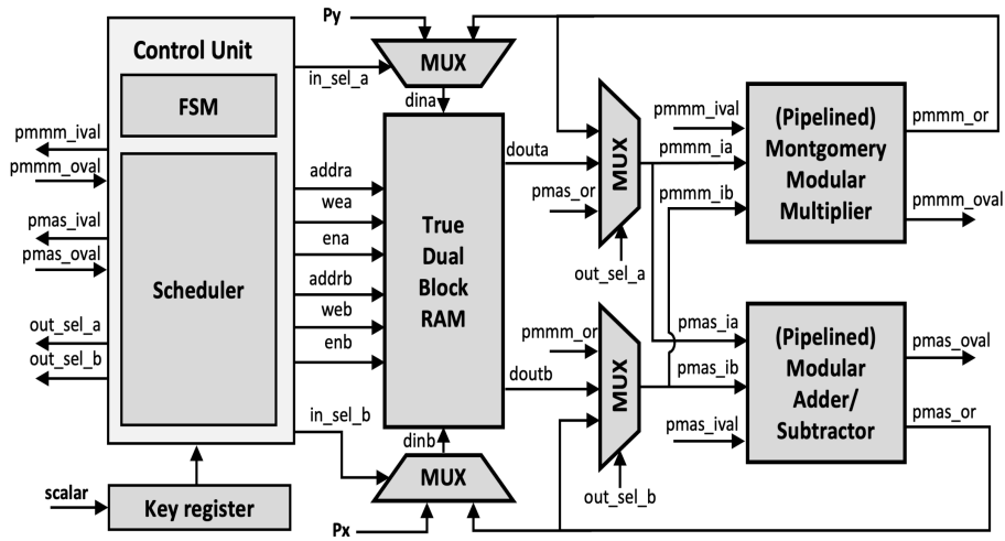
Figure 4.4: The elliptic curve cryptography (ECC) architecture proposed in article [11]. The figure is retrieved from [11].
