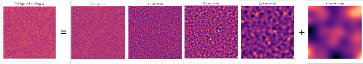
Figure 5.1: Visualisation of the starlet decomposition of an original noisy convergence map. The original noisy convergence map is obtained by applying shape noise to a noiseless realisation of the MassiveNus convergence maps products. Then by convolution with a 2D starlet, the original image is decomposed in several different images corresponding to the scale 2^j plus a smoother (coarse) version of it. Here we show the decomposition for a map of the fiducial cosmology. The resolution for the MassiveNus simulations convergence maps is \sim 0.4 arcmin.
