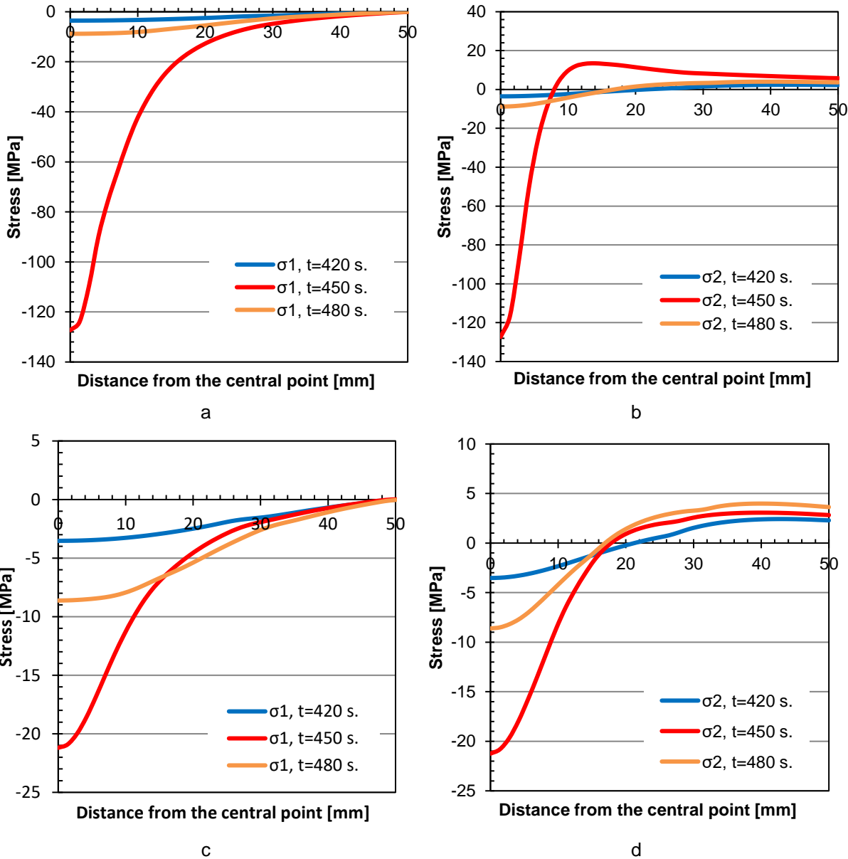
Figure 5-16. Stress distribution along sample radius developed at three relevant moments around the 5th cycle: just before heating (t=420 s.), at the end of heating (t=450 s.) and 30 seconds after heating (t=480 s.). a) The first principal stress (radial) at the top surface, b) the second principal stress (hoop) at the top surface, c) the first principal stress (radial) at the bottom surface, d) the second principal stress (hoop) at the bottom surface.
