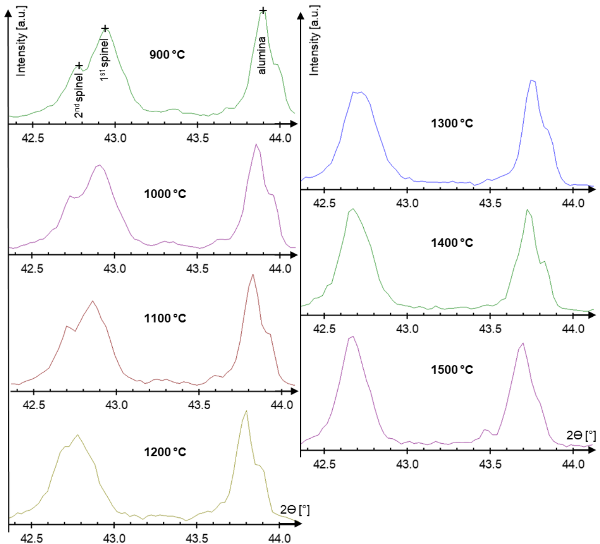
Figure 4-14. High-temperature X-ray diffraction diagram in the 2\theta angle range of 42.4-44.1^\circ aiming to compare an alumina peak from two spinel peaks for 12S6CMA-W-A castable.
