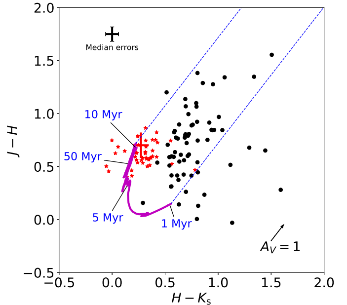
Fig. 2. Color-color diagram (J-H) versus (H-K_s) for the selected sample of SSCs (black dots). The theoretical stellar evolution track given by SB99 is shown for solar metallicity as the solid magenta line. The reddening vector corresponding to A_V = 1 is shown. The red stars are the sources detected in the control field, and the cross corresponds to the average color indices of the sample of 100 galaxies from the 2MASS survey, studied by Jarrett et al. (2003), with the length of the arms being equal to the standard deviations of those indices. The black cross represents the median errors of the cluster colors.
