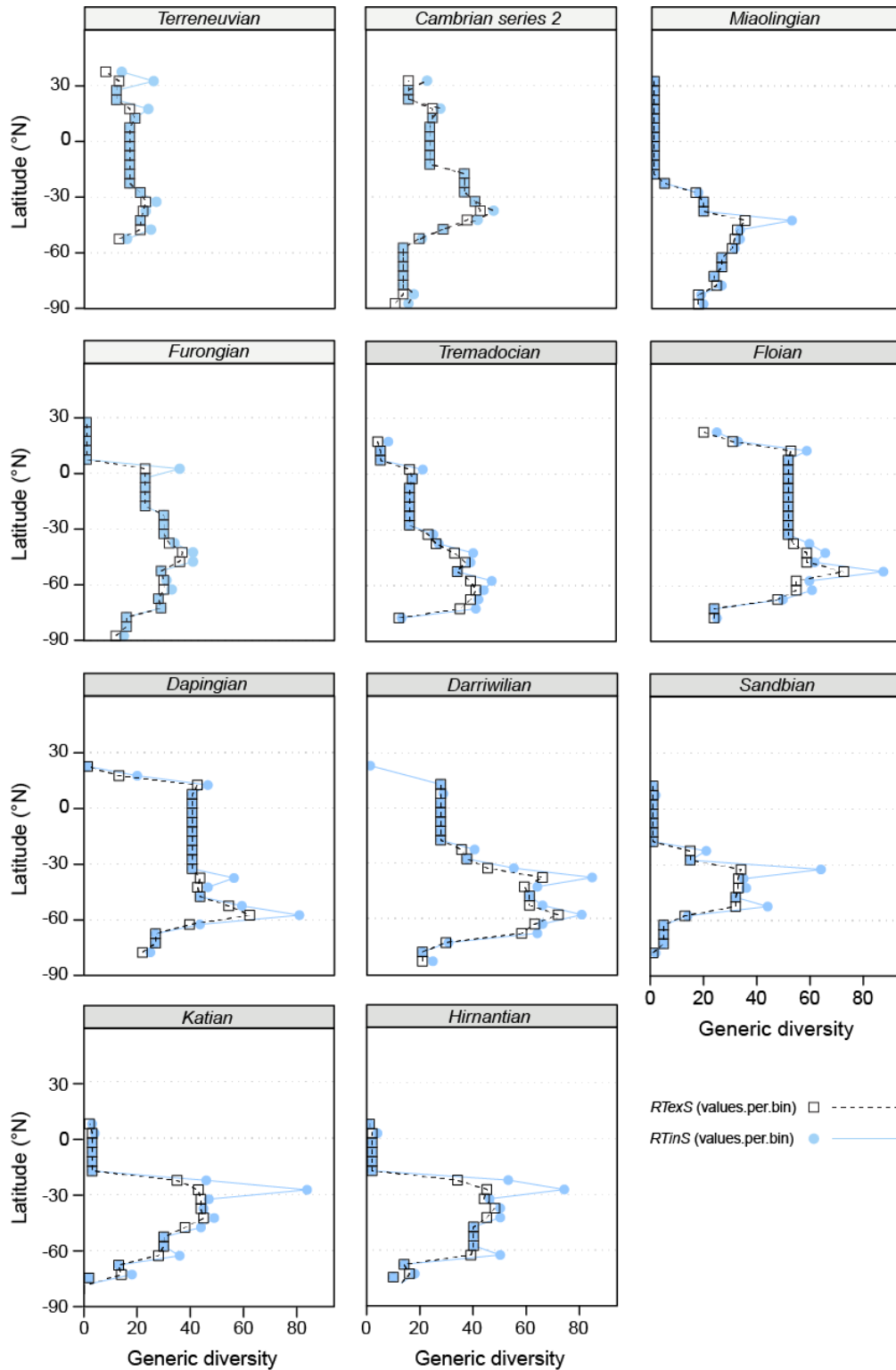
703 704 Figure S1. Acritarch genus diversity calculated per 5° latitudinal bands for each series of the Cambrian 705 and each stage of the Ordovician. Diversity was calculated using the standard ‘range-through’ counting 706 approach, with and without single-interval taxa ( RTinS and RTexS and indices, respectively).
