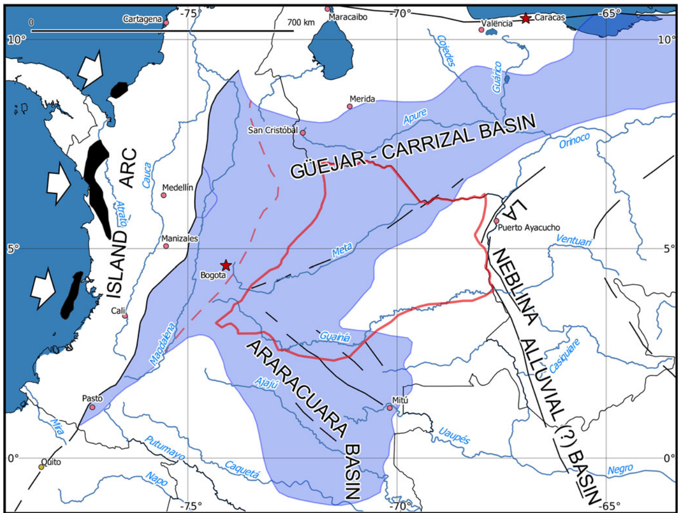
Figure 2. Depositional basins in north-western South America during the Cambrian–Ordovician. Dashed line: basement boundary between Chicamocha Terrane in the west and the Guyana Shield in the east. Based on Cediél et al. (2011).
