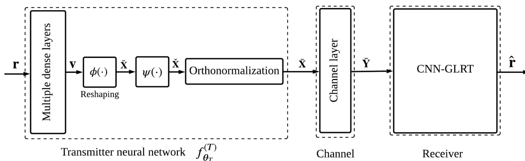
FIGURE 5.2 – Structure of the proposed AE-GLRT.
