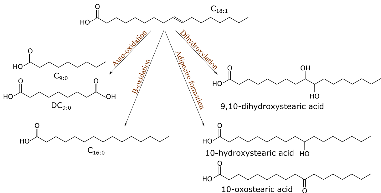
Figure 20. Main degradation pathways of fatty acids in archaeological context
