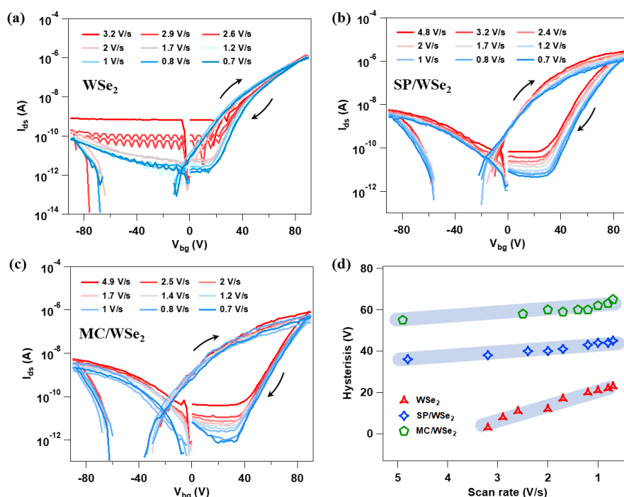
Figure 8-20. Hysteresis characterization of (a) bare WSe 2 , (b) SP/WSe 2 and (c) MC/WSe 2 FET under different scan rates, (d) Hysteresis comparison between the three conditions.
