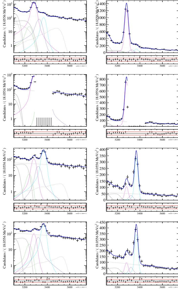
Figure B.2: Result of the simultaneous fit to the data. We show here the results on 2018, LL. The selection has been optimised on the principal signal peak. From top to bottom, K_S^0\pi^+\pi^- , K_S^0K^+K^- , K_S^0K^+\pi^- and K_S^0\pi^+K^- are shown. The left-hand-side plots have a logarithmic scale, and the plots on the right show the same data on a linear scale. The magenta dashed line is the B^0 signal contribution. The B_s^0 signal peak is in cyan. The crossfeed backgrounds are the blue and green dashed lines. The grey dashed line peaking above 5400 MeV is the \Lambda_b crossfeed background. To the left of the plot, the grey dashed lines illustrate the partially reconstructed background contributions and the combinatorial background is the grey straight line. In the K_S^0K^+K^- spectra, the region around the B_s^0 signal (5320-5450 MeV) is blinded.
