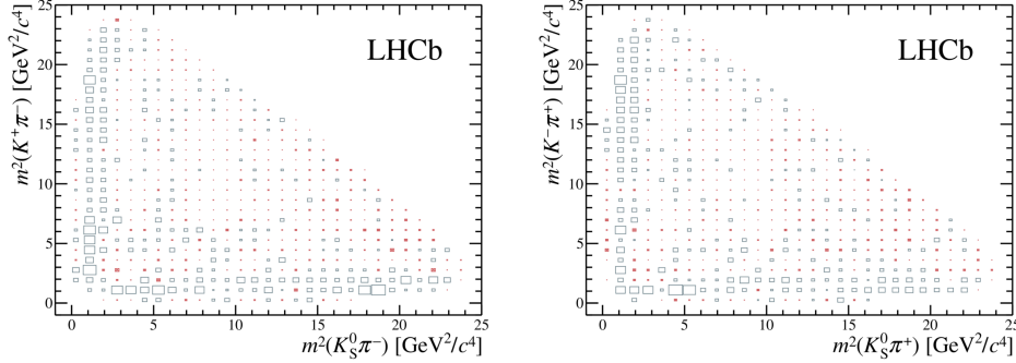
Figure II.4: Figure from an LHCb analysis of B_s^0 \rightarrow K_S^0 K^+ \pi^- showing the dalitz-plot distribution of the B_s^0 \rightarrow K_S^0 K^+ \pi^- signal events at the left and B_s^0 \rightarrow K_S^0 K^- \pi^+ at the right. The background contributions have been subtracted and the efficiency has been corrected thanks to the studies performed during the Run 1 K_S^0 h^+ h'^- analysis [9].
