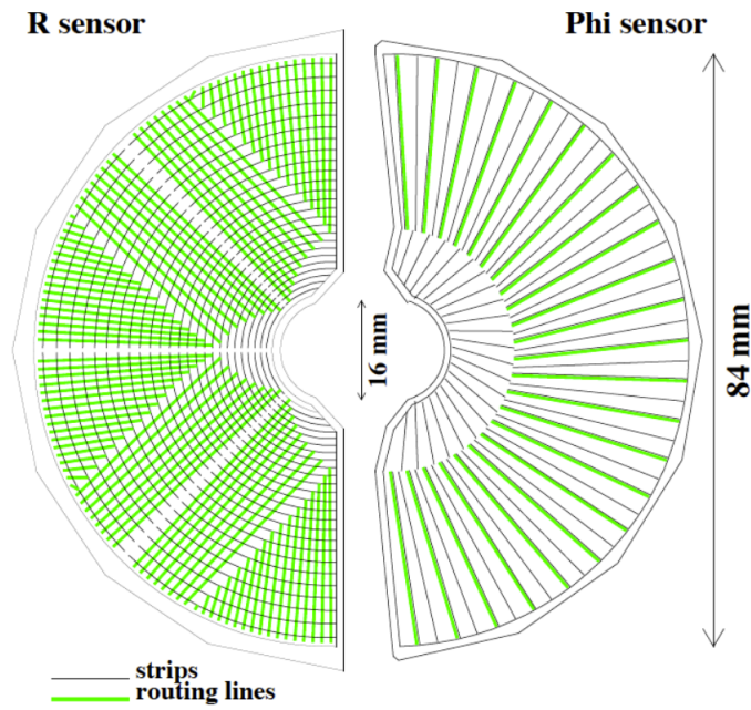
Figure IV.7: View of the \Phi and R sensors. [62]
