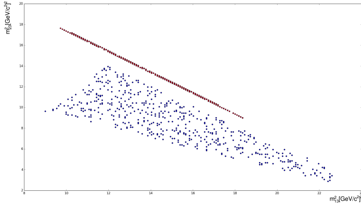
Figure III.4: I ran an algorithm to match together 2 points with correlation below 90%. We see that these points are chosen in the same kind of region - most of the time, one point is picked along a narrow resonance close to the edge of the Dalitz plane, the second point is then picked closer to the centre where the amplitude are usually quite low.
