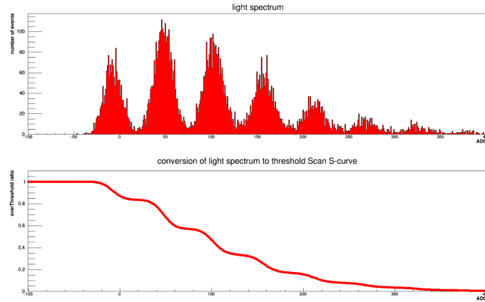
Figure V.5: Example of a light spectrum (top) and an S-curve (bottom) produced during a threshold scan. Threshold scans are performed in order to calibrate the PACIFIC module. Thanks to this calibration, we can obtain an equivalence between the ADC units and the number of photo-electron received from the SiPMs [82].
