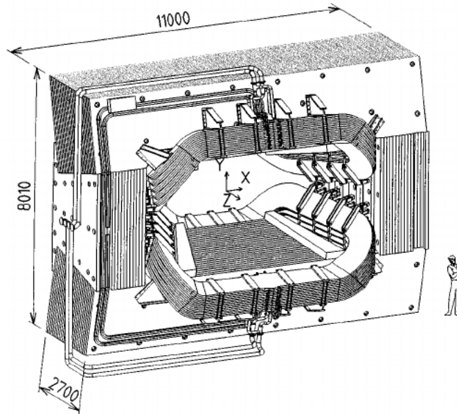
Figure IV.4: Schematics of the LHCb magnet.
