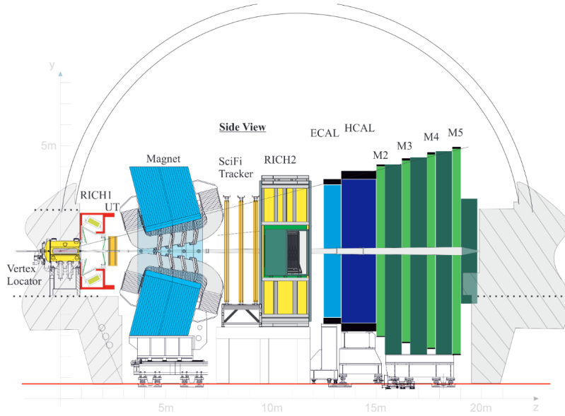
Figure V.2: Schematical view of the LHCb upgraded detector [80].
