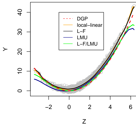
Figure 5.4: Comparison between nonparametric estimators
