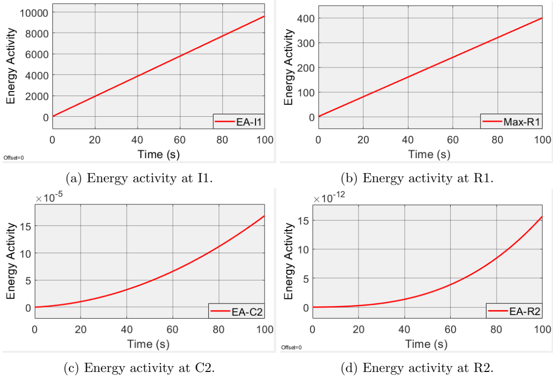
Figure 3.5: Energy Activity of elements in circuit.
