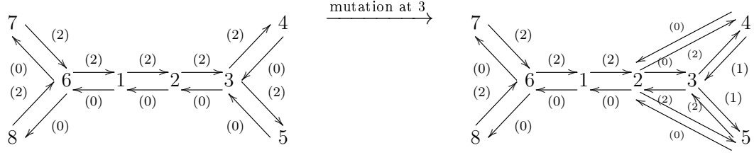
Figure 1.17 – Quiver mutation is compatible with the flip of an (m+2) -angulation, for m = 2 . In order to keep a clear figure, we have not replaced the arcs 8 and 5 by loops.
