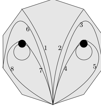
Figure 1.28 – The initial quadrangulation for n = 7 and m = 2
