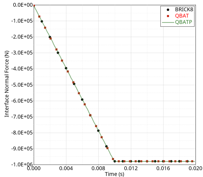
Figure 3.40: Test 3.9: Evolution of normal contact force (N)
