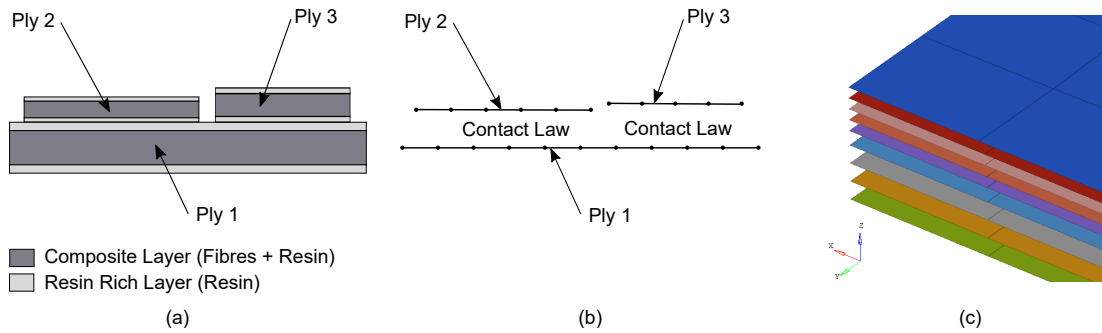
Figure 2.3: (a) Schematic representation of prepreg stack (b) Modeling strategy for prepreg stack for QSP ® in Altair Radioss ™ (c) Zoomed in view of the actual component with 9 plies modeled in Altair Radioss ™
