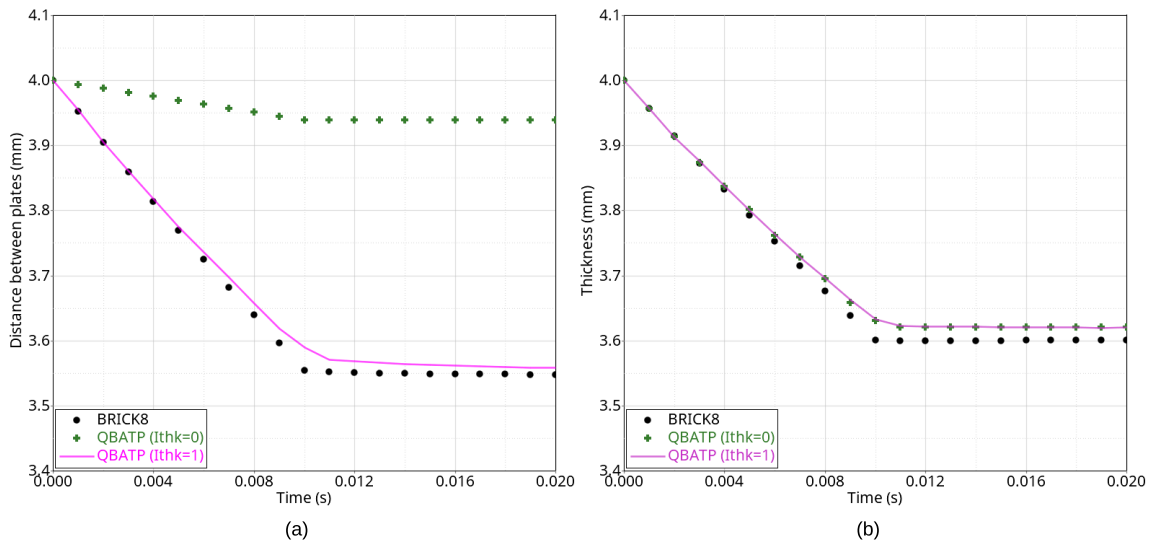
Figure 3.45: Test 3.9: Comparison of (a) distance reduction and (b) thickness evolution for BRICK8, QBATP without gap dynamic gap update and QBATP with dynamic gap update
