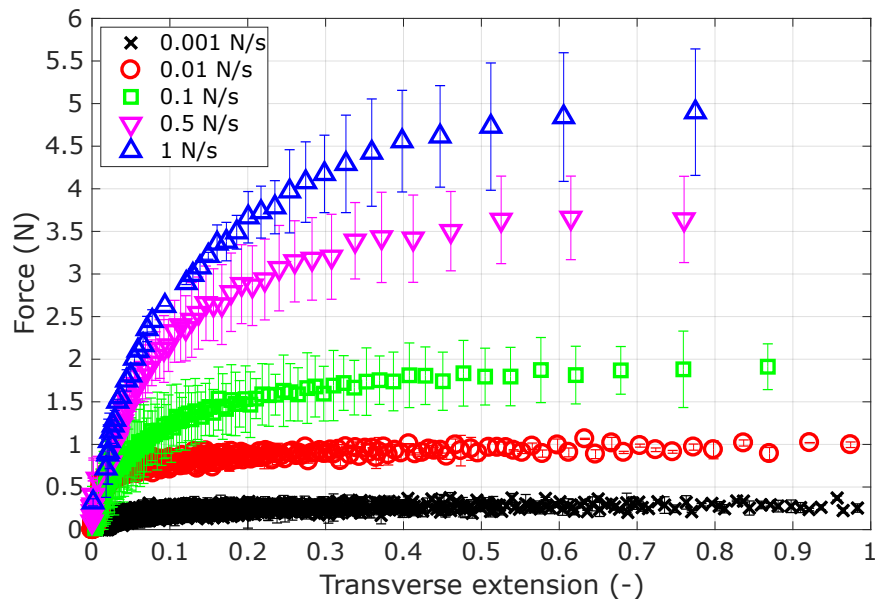
Figure 2.10: Quantitative results showing the raw force and displacement recorded for several force rates
