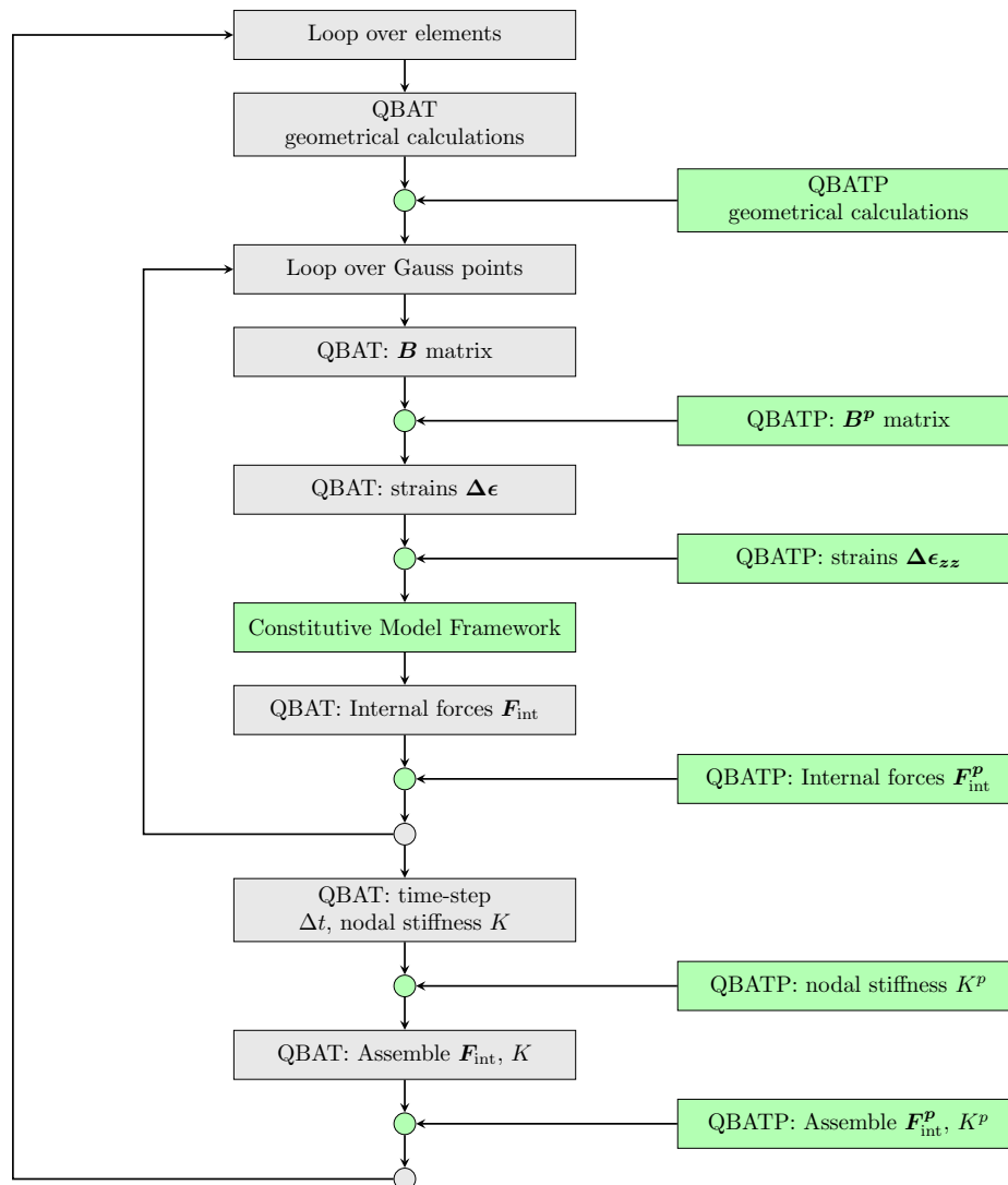
Figure 3.9: Overview of the F_{\text{int}} and F_{\text{int}}^p calculation (green colored boxes show the implemented framework in this work)
