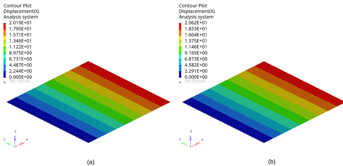
Figure 3.26: Test 3.5: Comparison of displacement field X (mm) (a) BRICK8 element (b) QBATP element
