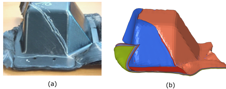
Figure 5.11: Comparison of final deformed shape (a) Experiment (b) Simulation with a unified approach
