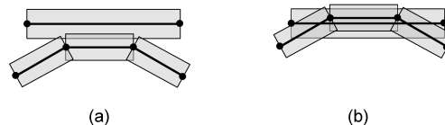
Figure 5.5: (a) Penetration (b) Intersection
