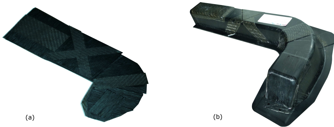
Figure 1.4: (a) Flat two dimensional stack of prepreps before QSP ® (b) Final formed part
