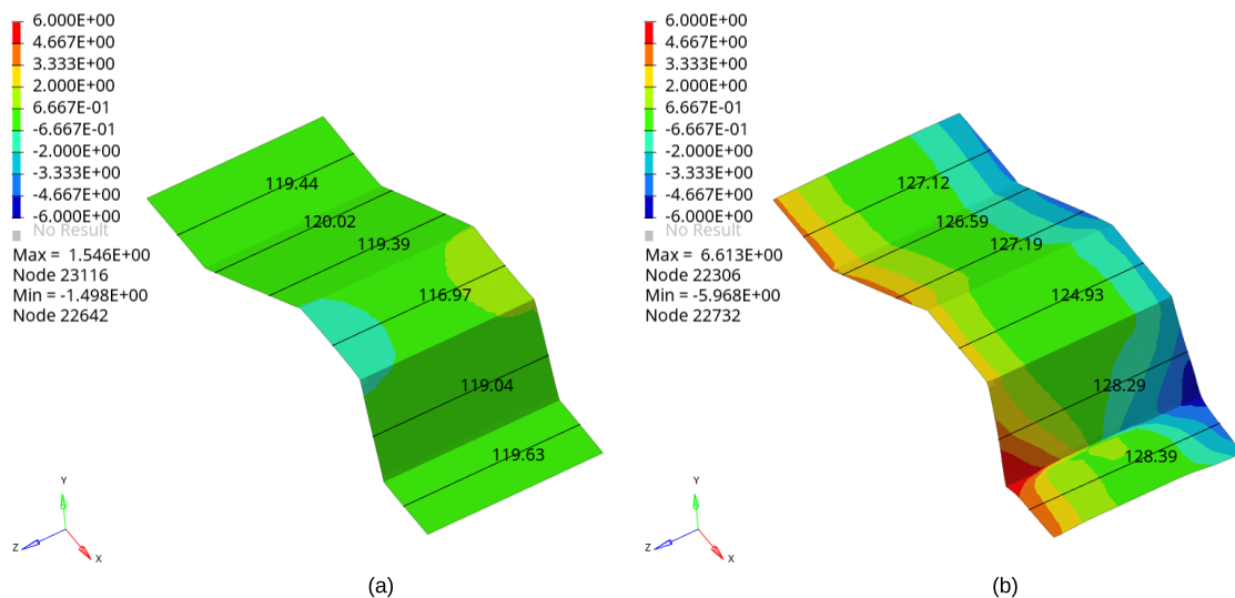
Figure 3.47: Forming and consolidation of a semi-industrial model: Comparison of displacement Z (mm) for (a) QBAT simulation (b) QBATP simulation
