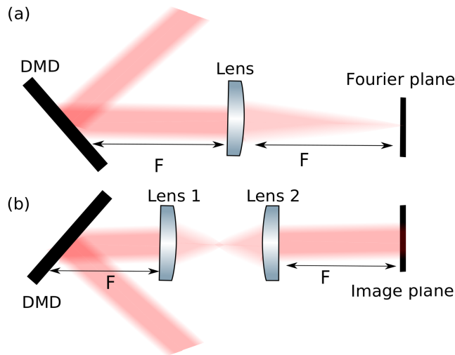
Fig. 3.7: Imaging configurations of DMD (a) Fourier plane of the DMD: The beam diffracted from the DMD is focussed in the Fourier plane of the lens shown. (b) Lens 1 focuses the incoming beam into a Fourier plane as above and then the lens 2 does the inverse-Fourier transformation of this beam to image the plane of the DMD pixels onto the plane of the image, where ultracold atoms are placed in the experiment [136].
