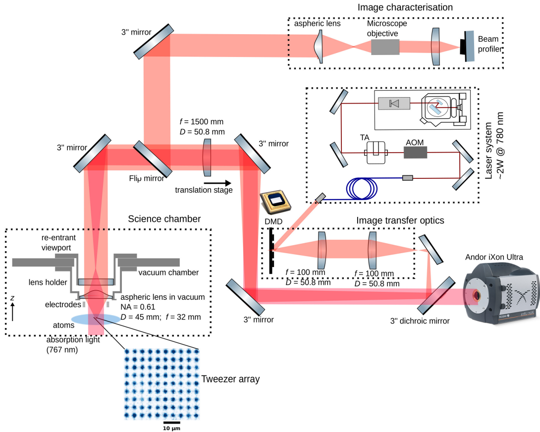
Fig. 3.8: Experimental setup showing the integration of DMD in the high resolution imaging system: The experimental setup shown above includes the imaging system for creating tweezer arrays consisting of Image transfer optics : DMD + two lenses of focal length 100 mm each forming a telescope with magnification = 1 then a lens with focal length of 1500 mm (situated on a translation stage) + an aspheric lens of focal length 32 mm inside the vacuum chamber (as shown in Science chamber ) has an effective magnification of \approx 53 . Hence, at the focus of this high resolution imaging system is a DMD pattern that is de-magnified by 53 times to project on to the atomic cloud trapped in optical dipole trap. An absorption shadow of the atoms from the tweezer traps is imaged onto a charge-coupled-device camera 9 using the same optics as for the DMD light patterns. The 780 nm laser system: The light used to create the microtraps is obtained from the ECDL laser at 780 nm and the power of the laser output is magnified to \approx 2 W using a tapered amplifier 12 . An AOM is used for fast switching of this trap-light. Image characterisation: This is a test-setup to characterise the tweezer trap patterns produced using DMD. Using a flip mirror after the lens of focal length 1500 mm, the trap beam of 780 nm is re-directed to an another aspheric lens (focal length of 32 mm) to de-magnify the DMD patterns by 53 times. The resulting image is then observed on the beam profiler 15 using a microscope objective 14 .
