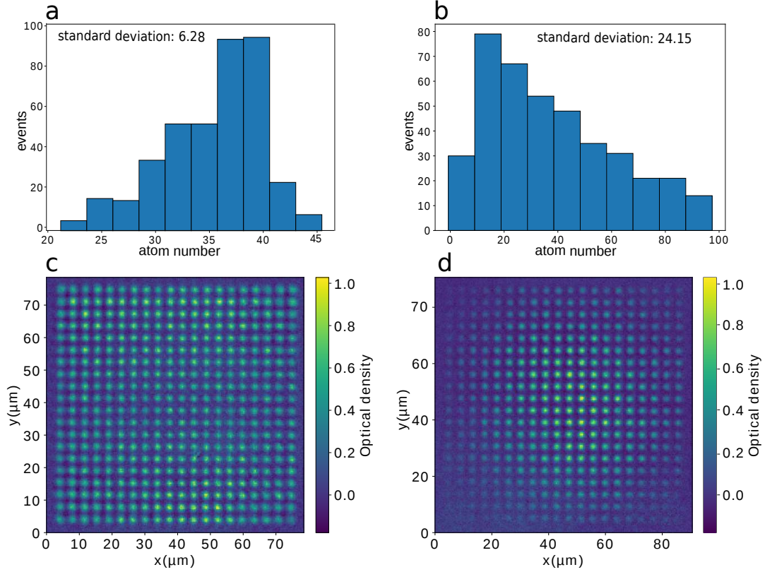
Fig. 4.6: Comparison of uniformity in atom loading into the array of tweezers produced using the DMD patterns with and without Gaussian gradient modification (a) and (b) are histograms of atom number extracted from the experimental absorption image shown in (c) and (d) respectively. (c) Experimental absorption image of a 400 site square lattice (averaged over 20 repetitions) produced using gradient (Gaussian) modified DMD pattern (see equation 4.8), where each spot corresponds to a microscopic ensemble of \approx 30 ultracold ^{39}\text{K} atoms. The lattice spacing is 3 \mu\text{m} and the apparent size of each spot is \sim 0.9 \mu\text{m} ( e^{-1/2} radius). (d) Experimental absorption image of a 400 site square lattice (averaged over 20 repetitions) produced without any gradient modification applied to DMD patterns. The lattice spacing is 4 \mu\text{m} . The standard deviation calculated from the average of 20 images is 0.17\langle\bar{N}\rangle_m as shown in (a), compared to 0.55\langle\bar{N}\rangle_m without any gradient modification as shown in (b). Hence, gradient modification of the DMD patterns increases the uniformity of atom loading into the tweezers by \approx 3 times.
