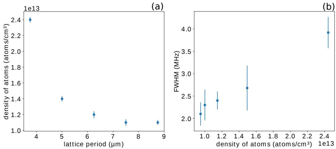
Fig. 5.9: Density effects on spectral broadening. (a) The atomic density in the tweezer traps increase with decrease in the lattice period where the adjacent atomic clouds start overlapping with each other. The error bars are the standard errors calculated by taking the average of atomic densities for an array of 100 site square tweezer traps as shown in the figure 5.8. (b) A full width half maximum is calculated from the Gaussian fit to the spectra of the tweezer traps of period 3.5 \mu\text{m} by varying atomic densities as shown in (a). We can clearly observe the increase in the spectral broadening due to increase in atomic density as the lattice period reduces.
