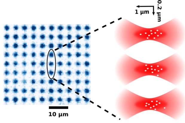
Fig. 2.1: Schematic representation of the array of optical dipole traps of atomic ensembles. In our experiments, the ensemble of atoms are confined within tweezer traps which are focused beams of Gaussian laser-light tuned far below atomic resonance separated by several micro-meters. Each blue dot in the array (left) represents an ensemble of \sim 40 atoms trapped in a focused laser beam. The separation between the adjacent blue dots is \sim 4 \mu\text{m} . On the right (zoomed-in), the illustration of ensembles of atoms trapped in focused laser beams has been shown.
