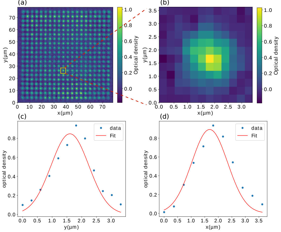
Fig. 4.2: Estimation of number of atoms in each tweezer. (a) Experimental absorption image of a 400 site square lattice, where each spot corresponds to a microscopic ensemble of \approx 30 ultracold ^{39}\text{K} atoms. The lattice spacing is 3.5 \mu\text{m} and the apparent size of each spot is \sim 1 \mu\text{m} ( e^{-1/2} radius) (b) Zoom-in of the marked spot. (c) Vertical-crosection of the marked spot with the fit of 2d Gaussian function. (d) Horizontal-crosection of the marked spot with the fit of 2d Gaussian function. By finding the fit results of \sigma_x, \sigma_y , we obtain the width of atomic cloud in x and y direction and the fit results of the amplitude of this function conveys the optical depth (OD) of the cloud. With these parameters, the number of atoms in each atomic cloud per tweezer are estimated (equation 4.5).
