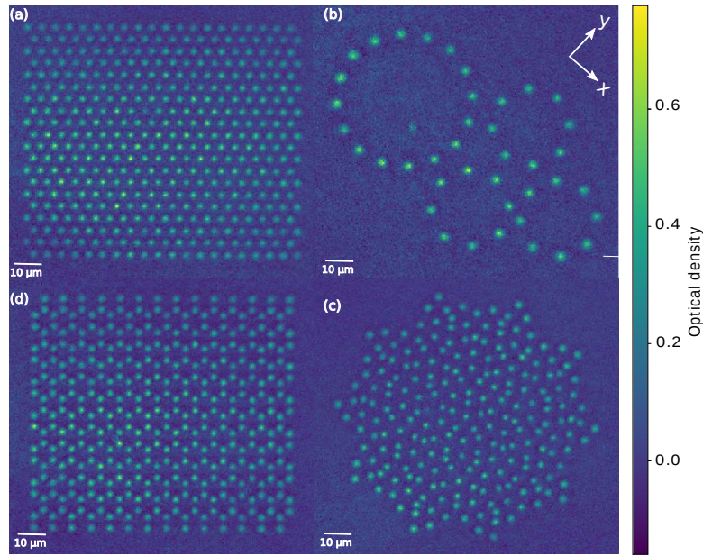
Fig. 4.1: Realization of large tweezer arrays with large occupation number in each tweezer. (a) Experimental absorption image of 400 site triangular lattice, where each spot corresponds to a microscopic ensemble of \approx 30 ultracold ^{39}\text{K} atoms. The lattice spacing is 4 \mu\text{m} and the apparent size of each spot is \sim 0.75 \mu\text{m} ( e^{-1/2} radius), mostly limited by recoil blurring during imaging. (b) 40 site ring structure (c) 226 site Penrose quasicrystal lattice. To improve the signal-to-noise ratio each image is an average of 20 absorption images (d) 196 site honeycomb lattice (see figure 4.3a for a typical single shot image).
