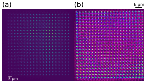
Fig. 3.12: Intensity profiles with and without Gaussian compensation. (a) An intensity profile observed on a beam profiler 15 created by DMD without using any Gaussian compensation i.e. parameter 'g' = 0. This image shows a 20 \times 20 square lattice with lattice period of 5 \mu\text{m} . (b) An intensity profile of 22 \times 22 square lattice created by DMD using the Gaussian compensation with A_{min} = 20 pixels and the parameter 'g' = 1.2 and the lattice period of 3 \mu\text{m} .
