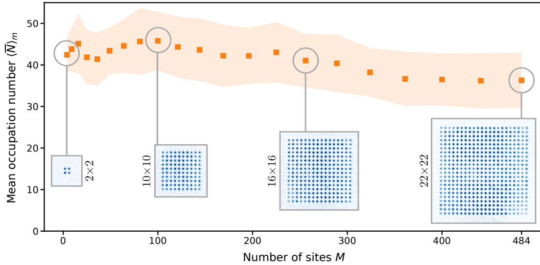
Fig. 4.5: Scaling up to hundreds of tweezers. The square data points show the array-averaged mean occupation number for square arrays with a period of 3.5 \mu\text{m} and different numbers of sites ranging from M = 2 \times 2 to M = 22 \times 22 . Over this range the array averaged occupation number \langle \bar{N} \rangle_m \approx 40 is mostly homogeneous and insensitive to the number of tweezers. The shaded region represents the uniformity of each array, computed as the standard deviation of the mean occupation number. The insets show exemplary absorption images for 4 different sized arrays, each averaged over 20 experimental repetitions.
