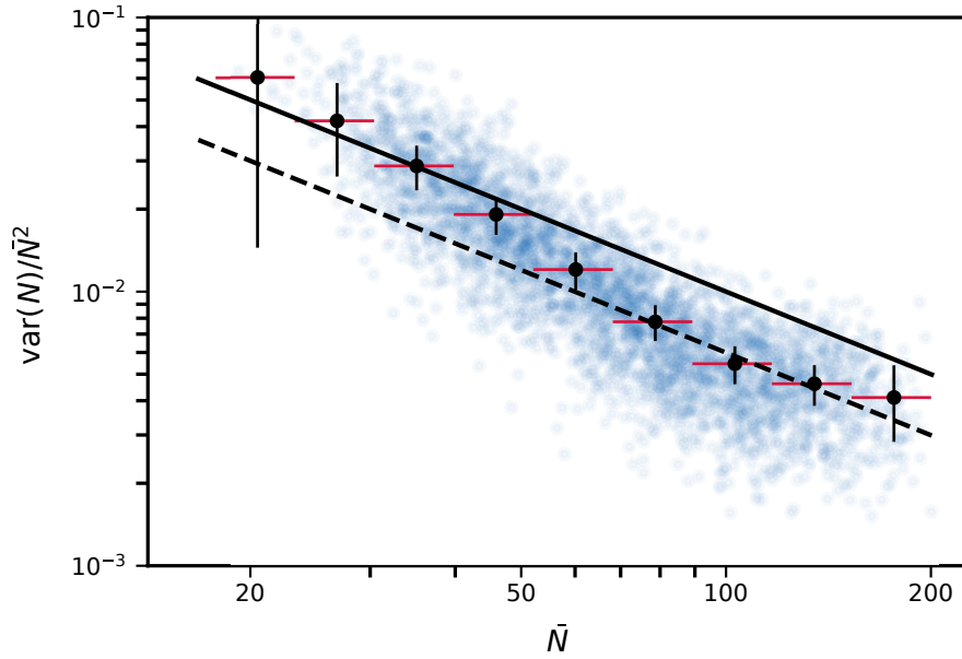
Fig. 4.8: Relative variance of the atom number in each tweezer \text{var}(N)/\bar{N}^2 as a function of the mean occupation number \bar{N} . The blue points show the relative variance computed from 20 repetitions of the experiment and for different mean occupation numbers. The black symbols show the same data after binning, where the bin widths are indicated by the horizontal red bars. The vertical error-bars show the standard error computed over the values inside each bin multiplied by a scaling factor of 10 for better visibility. The solid black line is a prediction assuming Poissonian atom number fluctuations \text{var}(N)/\bar{N}^2 = 1/\bar{N} and the dashed black line is a prediction assuming sub-Poissonian atom number fluctuations \text{var}(N)/\bar{N}^2 = 0.6/\bar{N} .
