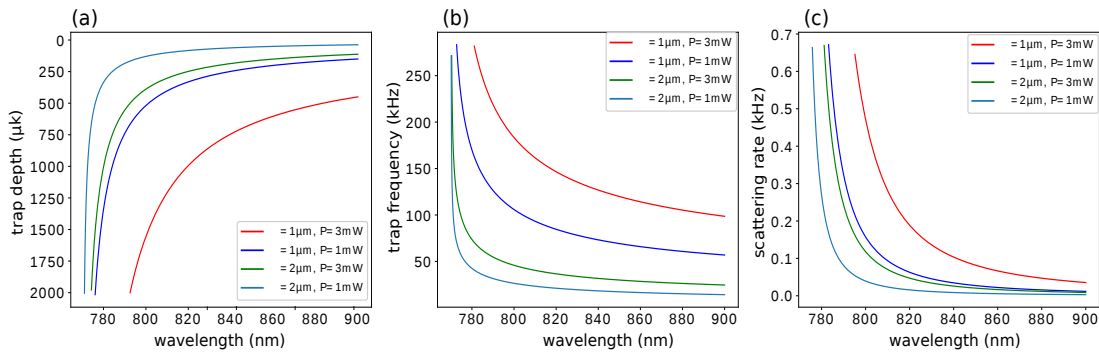
Fig. 3.14: Estimation of microtrap parameters. We make the choice of trap-wavelength of 780 nm to generate microtraps. From figure (a), we can see that the trap depth at 780 nm is \approx 1 mK and trap-frequency of around 100 kHz, (figure (b)) which belongs to the beam waist in between 1-2 \mu\text{m} as the optical resolution is \approx 1 \mu\text{m} (see figure 3.10) and power of around 1-2 mW as power efficiency of DMD is only a few percent of the incident power of the laser light [135] but a relatively higher photon scattering rate (figure (c)).
