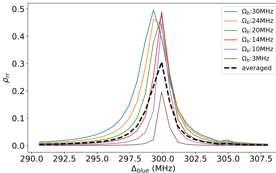
Fig. 5.7: Simulation of three-level Optical Bloch Equations for different Rabi frequencies of the upper transition: This figure represents the excited state population calculated using the quantum master equation from chapter 2 section 2.2.1 at steady state. Using the detuning of the lower transition (-300 MHz), two-photon resonance is achieved for an upper state detuning \delta = 300 MHz. The different curves correspond to the different Rabi frequencies for the upper transition ( \Omega_b ), from 30 MHz to 3 MHz. The position of the peak shifts due to the AC stark shift of the upper transition \Omega_b^2/2\Delta [107]. Each spectral line has a width of \approx 2 MHz. The little bump on the right is an artifact of the numerical calculation.
