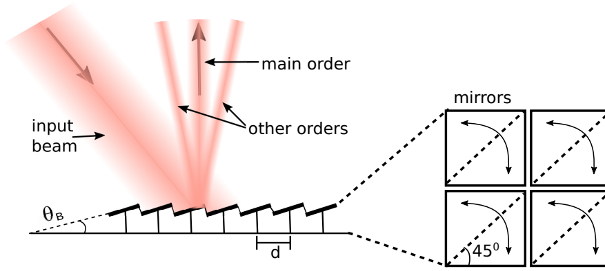
Fig. 3.6: DMD as a blazed grating The DMD mirrors constitute a blazed grating [136, 137]. Hence, an incident beam gets diffracted in different orders. Depending on the mirror spacing d , the mirror tilt angle and the wavelength of the laser light, a main order carries most of the reflected intensity and the other orders carry less. These mirrors tilt about its diagonal axis. The DMD should be mounted at 45^\circ to keep the reflected laser beams in the same horizontal plane as that of the optical table.
