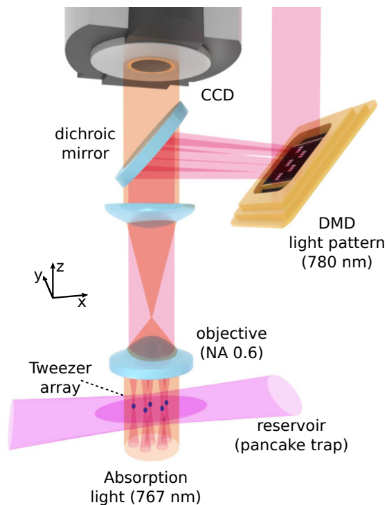
Fig. 1.2: Schematic of the setup from our lab in Strasbourg used to produce and load the tweezer arrays by projecting light from a digital micromirror device directly onto the atoms confined in an optical reservoir trap.
