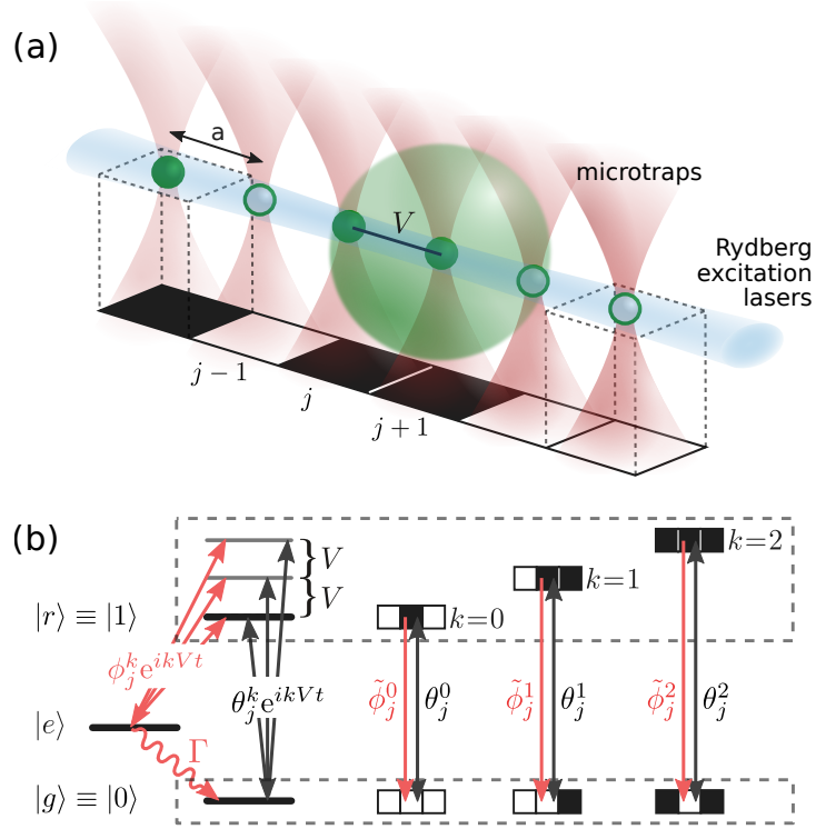
Fig. 6.3: Physical platform for quantum cellular automata based on arrays of Rydberg atoms: (Image reproduced from [96]) (a) Proposed setup showing a 1D array of atoms held in optical microtraps with period a and nearest-neighbor Rydberg-Rydberg interaction strength V . (b) Each atom can be described as a three-state system: |g_i\rangle (open symbols) |r_i\rangle (solid symbols) and an additional short lived state |e_i\rangle . The |g_i\rangle to |r_i\rangle and |r_i\rangle to |e_i\rangle transitions on site j are coupled by multifrequency fields with detunings kV and coupling strengths \theta_j^k and \phi_j^k respectively. This system can be reduced to an effective two-state system with programmable K -body interactions (shown on the right for K = 3 ) where the couplings \theta_j^k and \tilde{\phi}_j^k realize unitary (reversible) and non-unitary (dissipative) conditional interactions dependent on the number of excited neighbors k .
