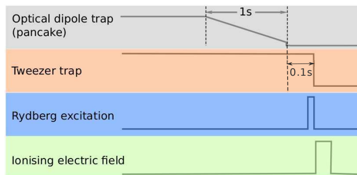
Fig. 5.5: Sequence of spectroscopic measurements from atoms trapped within the array of tweezer traps: The pancake trap power is ramped down during the atom-loading from pancake trap to the array of tweezer traps. The pancake trap is switched off for 100 ms before the Rydberg excitation pulse to avoid any excitation signal coming from background atoms from pancake trap. The tweezer trap stays on during Rydberg excitation pulse. We use the 767 nm light in addition with the blue light (457 nm) for Rydberg excitation. The excitation pulse length is 100 \mu\text{s} . The final Rydberg atom number is detected via electric field ionisation. The sequence is repeated for different detunings \delta of the blue light from the Rydberg transition 69S_{1/2} .
