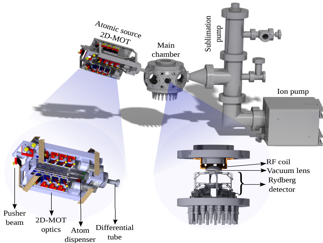
Fig. 3.1: Overview of the experimental apparatus. (Image reproduced from [111]) The main parts in the experimental setup are represented in here. The potassium dispenser-atom source (left) is placed inside a glass cell, and the surrounded optics constitute the 2D MOT (see zoom in) that creates a stream of atoms cold in the transversal directions that gets pushed towards the main chamber (center in the figure). The atoms go through a differential tube into the main chamber where they get further cooled and trapped. Inside the chamber a high resolution imaging lens, an MCP Rydberg ion detector and a radio-frequency antenna are placed for manipulation and state control. To maintain the high vacuum in the chamber, we have the ion pump and the sublimation pump on the right to the main vacuum chamber. Image adapted from [111]
