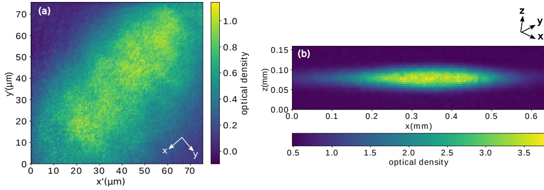
Fig. 3.4: Absorption image of ^{39}\text{K} in a pancake-shaped optical dipole trap: Atoms are loaded into the pancake-shaped optical dipole trap from the compressed MOT during the cooling stage through gray molasses. (a) High-resolution absorption image of the atom cloud trapped in the pancake shaped optical dipole trap. The image is taken from the top along the z axis. (b) Side absorption image of the atom cloud trapped in the pancake shaped optical dipole trap at the end of a time of flight. The image is taken along the y axis.
