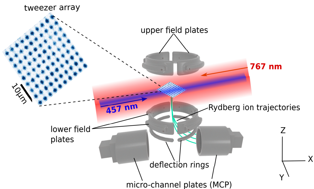
Fig. 5.1: Excitation laser setup to create Rydberg atoms: Schematic of counter-propagating two-photon excitation laser beams 767 nm (red arrow) + 457 nm (blue arrow) around the vacuum chamber to create Rydberg excitation in the microscopic atomic ensembles that are trapped within the large arrays of tweezer traps at the center of the vacuum chamber. The Rydberg detector assembly is composed of two sets of four electric field plates each, placed above and below the atomic cloud, that compensate the stray electric fields during Rydberg excitation and perform the ionization of the Rydberg states by the application of large voltages. The ions travel towards a micro-channel plate (MCP) detector by following the corresponding fields produced by the deflection rings (the trajectory of ions is shown using the green arrow). Figure modified from [134].
