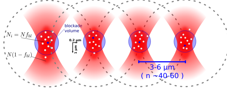
Fig. 4.7: Small spatial extent of microtraps The figure shows an array of 4 tweezer traps indicating the small spatial extent of tweezer trap of 1 \mu\text{m} in weak axis (z-axis) and 0.2 \mu\text{m} in tight axis. This small spatial extent of micro-trap lies well within the Rydberg blockade radius if the principle quantum number ( n ) = 40-60. The fraction of blocked atoms are shown as Nf_{bl} and the fraction of unblocked atoms are N(1 - f_{bl}) (equation 4.15).
