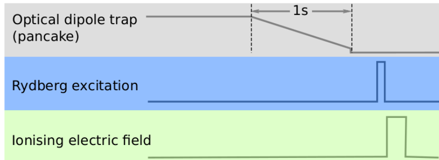
Fig. 5.3: Sequence of spectroscopic measurements from atoms trapped inside pancake-shaped optical dipole trap: The atoms are cooled down using evaporative cooling of the dipole trap. In these experiments, we use the 767 nm light plus the blue light to perform the Rydberg excitation. The excitation pulse length is 100 \mu\text{s} . The pancake trap stays on during the excitation to trap the atoms. The final Rydberg atom number is detected via electric field ionisation. The sequence is repeated for different detunings \delta of the blue light around the Rydberg transition 69\text{S}_{1/2} . This approach is similar to the one in [117].
