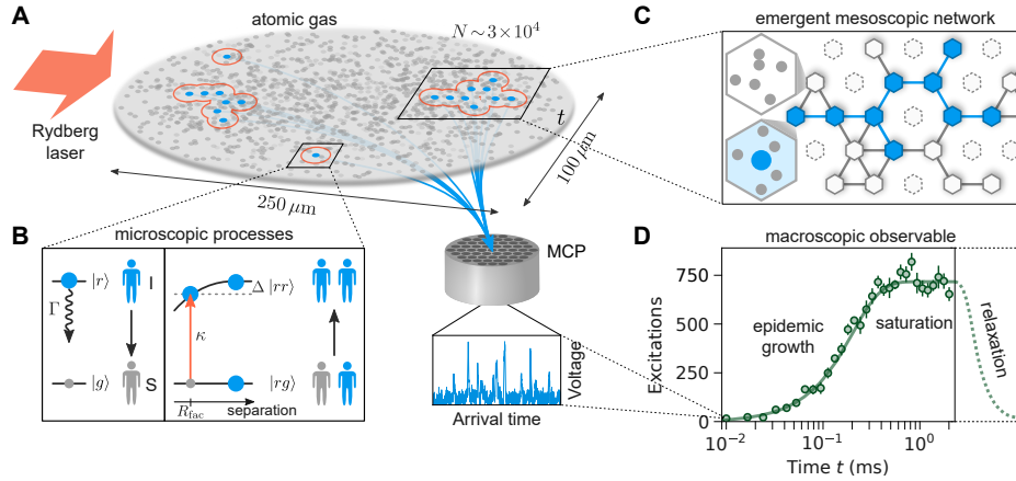
Fig. 6.1: Physical system for studying epidemic growth and dynamics on complex networks: (Image reproduced from [97]) (A) Experiments are performed on a two-dimensional continuous non-structured gas of potassium-39 atoms driven by an off-resonant laser field. The gas is initially prepared with a small number of seed excitations (blue disks) which then evolves according to the microscopic processes depicted in B, giving rise to growing excitation clusters that spread throughout the system. After different exposure times t , the Rydberg atoms are field ionized and detected on a microchannel plate detector (MCP), where the incident ions create voltage spikes (blue trace). (B) Each atom can be treated as a two-level system with a ground state |g_i\rangle (gray disks) and excited Rydberg state |r_i\rangle (larger blue disks). Excited atoms can decay with rate \Gamma or facilitate additional excitations with rate \kappa at a characteristic distance R_{\text{fac}} analogous to the transmission of an infection. (C) The dynamics of this system can be described by a susceptible-infected-susceptible (SIS) model on an emergent heterogeneous network. Each node represents a discrete cell of the coarse grained system, which can be infected (with excitation, blue) or susceptible (without excitation, white). The infection probability of each node is weighted by the number of atoms in that cell that can undergo facilitated excitation (disconnected nodes corresponding to vacant cells are depicted with dashed lines). (D) Exemplary data and numerical simulations (solid line) showing three different stages of dynamics: rapid growth, saturation, and eventual relaxation (data not shown). Error bars represent the standard error of the mean over typically 16 experiment repetitions.
