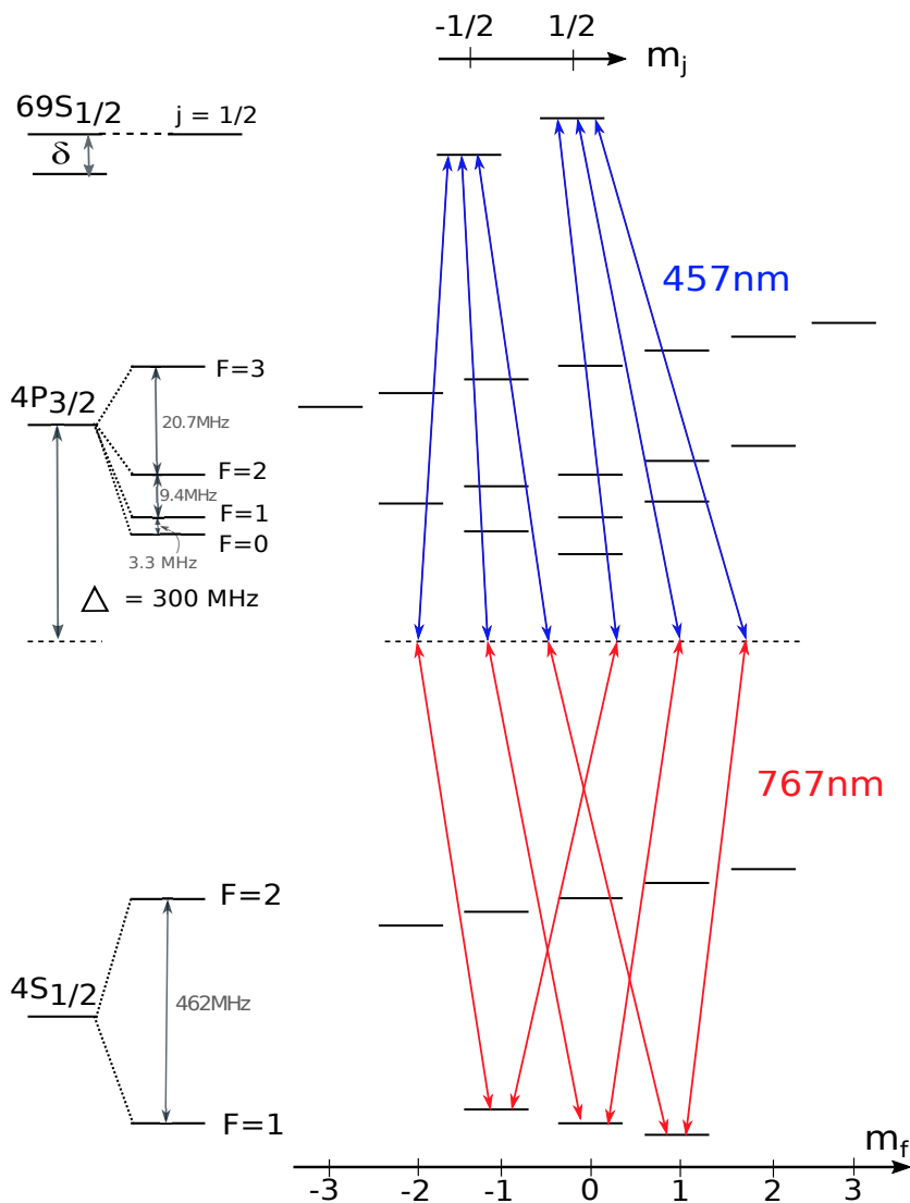
Fig. 5.2: Level schematic for two-photon Rydberg excitation: (Image reproduced from [117]) Level schematic for two-photon Rydberg excitation in a weak magnetic field. Atoms are prepared in the F = 1 , m_F = 0, \pm 1 ground states and are then excited to the Rydberg state 69S_{1/2} , m_j = \pm 0.5 via a two-photon transition, that is far detuned from the intermediate state by \approx 300 MHz. A linear Zeeman shift is induced for the m_f and the m_j levels by a weak magnetic field, resulting in six transitions.
