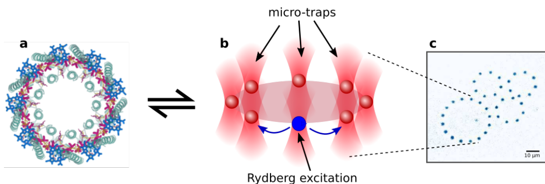
Fig. 6.2: Schematic representation of energy transport via Rydberg excitation hopping: (a) Molecular structure of the LH2 complex showing the ring-like arrangement of chromophores (hopping sites). (b) Proposed set-up of tweezer traps to simulate energy transport with controllable geometry (c) Experimental absorption image of a 40 site ring lattice structure, where each dark spot corresponds to a microscopic ensemble of \approx 30 ultracold ^{39}\text{K} atoms. The lattice spacing is 4\ \mu\text{m} and the apparent size of each spot is \sim 0.75\ \mu\text{m} ( e^{-1/2} radius), mostly limited by recoil blurring during imaging (reproduced from [51]).
