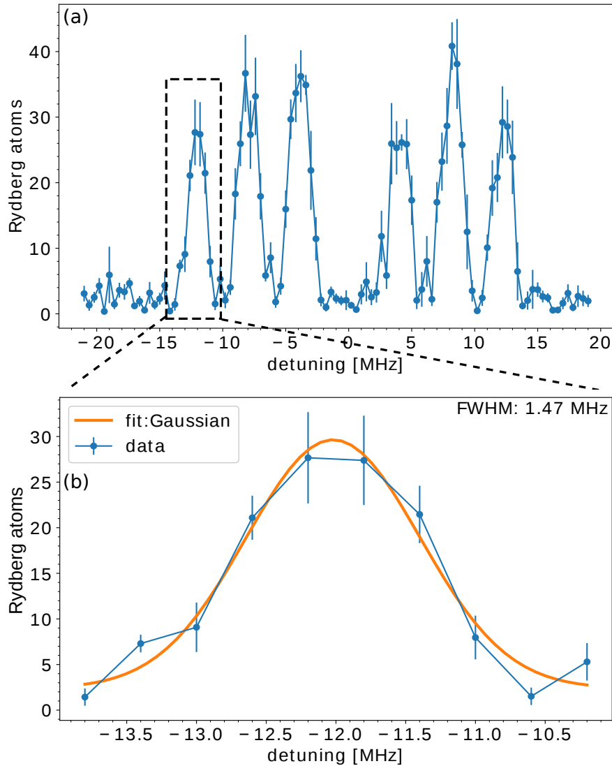
Fig. 5.6: Spectroscopic measurements of Rydberg excitation from atoms confined in tweezer traps: (a) Two-photon Rydberg excitation spectrum of atoms from array of tweezer traps obtained by scanning the detuning (x-axis) of the blue light (457 nm) across the Rydberg state 69S_{1/2} . The spectrum contains six peaks that represent the Zeeman splitting of the corresponding energy transition of 4S_{1/2} to 69S_{1/2} via the intermediate state 4P_{3/2} as described in figure 5.2. (b) The zoom-in of one of the peaks from the spectrum to determine the spectral width of the transition. A full width half maximum (FWHM) of the Gaussian fit to this peak estimates the spectral width of the corresponding transition which is 1.47 \text{ MHz} \pm 0.14 \text{ MHz} . These measurements are averaged over 5 repetitions and the error bars represent the standard error of the mean.
