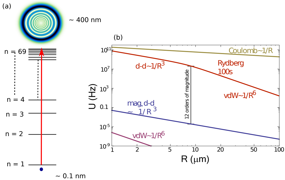
Fig. 2.2: Visualisation of giant size of Rydberg atom and interaction strength between two Rydberg atoms compared to the ground state atoms and the ions. (a) Rydberg atoms are atoms with their valence electron is excited to higher principal quantum number. They possess enormous dipole moment which results in the giant atomic size of n = 69 compared to the ground state atoms by 3 orders of magnitude. (b) (reproduced from [109]) This plot shows the interaction strength versus the distance between the two ground state atoms compared to the excited atoms to the 100s states and the ions. The interaction between two Rydberg atoms is \approx 12 orders of magnitude larger than between the ground state atoms.
