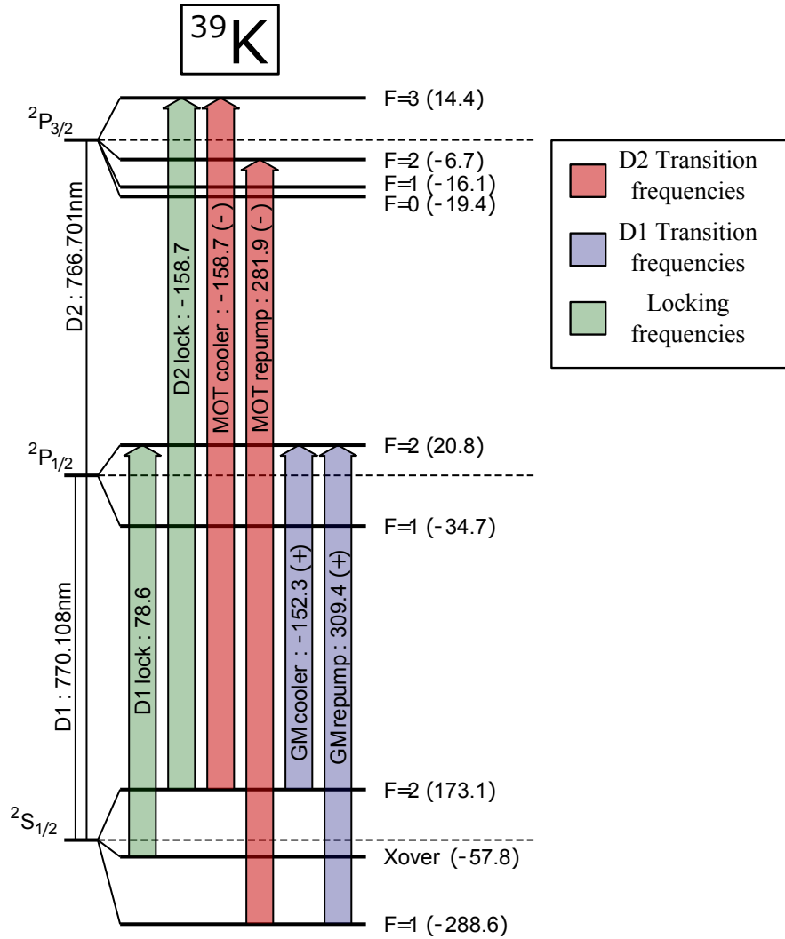
Fig. 3.2: Level scheme of potassium 39 and laser beam frequencies for the MOT and for the gray molasses. (Image reproduced from [111]) Two main transitions D1 and D2 transitions in ^{39}\text{K} respectively: |4S_{1/2}\rangle \rightarrow |4P_{1/2}\rangle and |4S_{1/2}\rangle \rightarrow |4P_{3/2}\rangle are represented with their corresponding hyperfine splitting. The blue arrows depict the cooling and repumping beam for the D1 transition while the red arrows represent the cooling and repumping beam frequencies for the D2 transition. The green arrows show the two frequencies (for the D1 and D2) that are used for locking the two lasers to the spectroscopy signal. Figure adapted from [120, 121]
