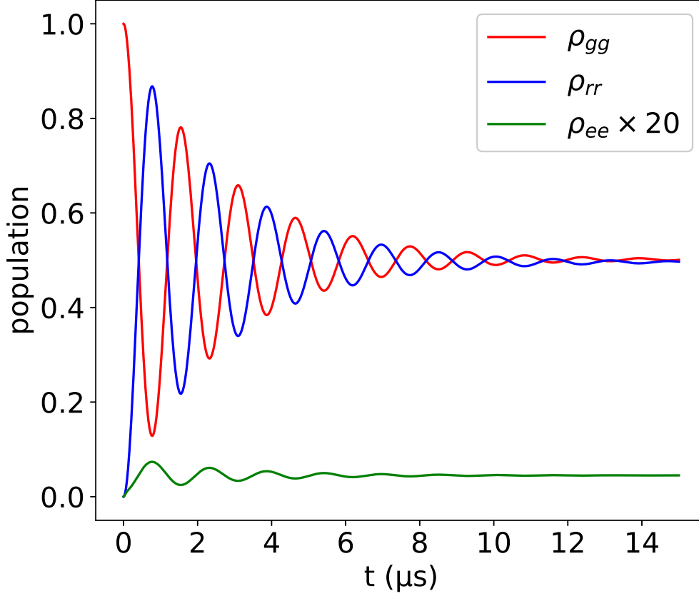
Fig. 2.4: Simulation of three level optical Bloch equations describing the time-evolution of the atomic system Population dynamics of ground state \rho_{gg} shown in red, of intermediate state \rho_{ee} shown in green and of Rydberg state \rho_{rr} shown in blue. The intermediate state detuning \Delta_1 = -300 MHz and the detuning with respect to the Rydberg state \Delta_2 = 300 MHz. At such a high detuning, the three level system effectively behaves as a two level system where population oscillates in between ground state and the Rydberg state without populating the intermediate state. Here \Omega_1 = 2\pi \times 13 MHz and \Omega_2 = 2\pi \times 30 MHz. The spontaneous decay rate from the intermediate state is equal to 2\pi \times 6 MHz which is equal to that of the D2 transition of potassium-39 and that of the Rydberg state is \sim 10 kHz. The laser linewidths \gamma_1 = 20 kHz and \gamma_2 = 60 kHz. All these parameters are similar to our actual experimental parameters. The condition of two-photon resonance is met as \Delta_1 + \Delta_2 = 0 . As we observe in the figure that the Rabi oscillations decay at \approx 15 \mu\text{s} . The effective Rabi coupling of this three level system \frac{\Omega_1\Omega_2}{2\Delta} is \approx 2\pi \times 0.63 MHz.
