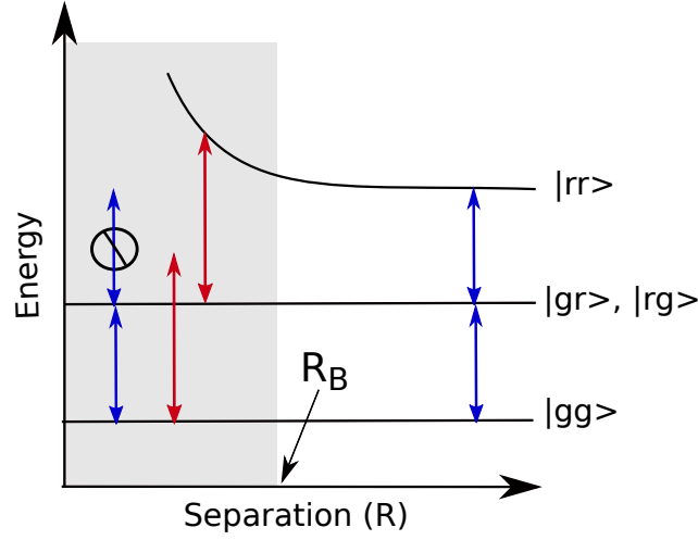
Fig. 2.5: Illustration of Rydberg blockade and anti-blockade effects. When the laser field is resonant with the Rydberg state (blue), an another Rydberg excitation is suppressed within the distance of the blockade radius R_B . The grey region represents the blockade area. At off-resonant laser frequency with respect to the Rydberg transition, an another Rydberg excitation can happen at a certain distance when the detuning is matched with energy shift of the Rydberg state.
