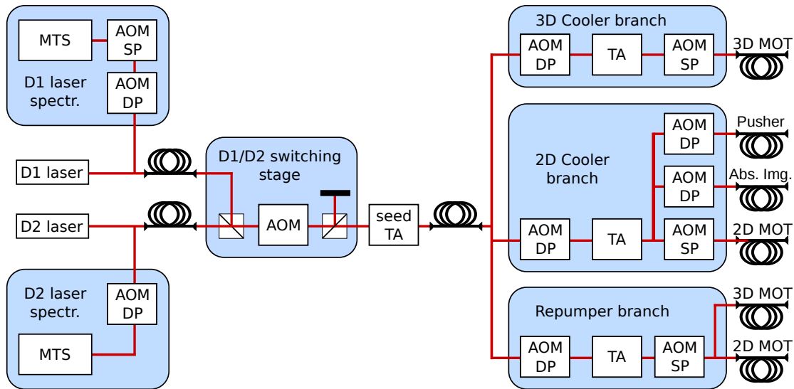
Fig. 3.3: A compact and versatile laser system for cooling and trapping. A schematic of the beam distribution of the laser system and the power amplification with all the necessary components such as tapered amplifiers, diode lasers and acousto-optical modulators for cooling and trapping in magneto optical trap (MOT). Image adapted from [121].
