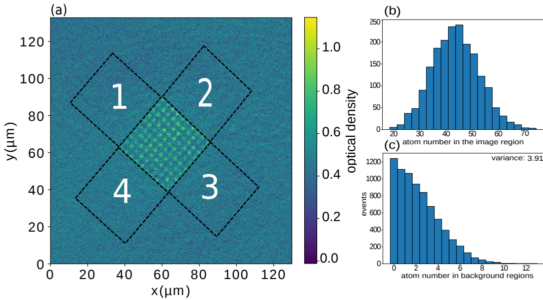
Fig. 4.3: Estimation of single shot detection sensitivity (a) Experimental absorption image of a 100 site square lattice, where each spot corresponds to a microscopic ensemble of \approx 40 ultracold ^{39}\text{K} atoms. The lattice spacing is \sim 4 \mu\text{m} and the apparent size of each spot is \sim 0.74 \mu\text{m} ( e^{-1/2} radius). Regions 1, 2, 3 and 4 are the background regions of interest to estimate the single shot detection sensitivity of 3.9 atoms as explained in section 4.1.2. (b) Histogram of estimated atom number distribution in the image region. (c) Histogram of estimated atom number distribution in the background regions 1, 2, 3, 4 where the variance is 3.91 atoms.
