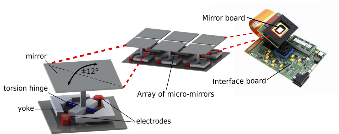
Fig. 3.5: Schematic of DMD Digital micromirror device where all of the 1024 \times 768 mirrors are situated on a rectangular mirror board of about 1.5 \text{ cm}^2 along with the zoomed-in part of the mirror array showing their tilt of \pm 12^\circ across the diagonal axis of the micromirror referring to the ON/OFF state of the device (Image adapted from [135, 136])
