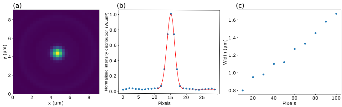
Fig. 3.10: Point spread function and intensity profile width of the DMD clusters with different pixels (a) The point spread function of the single pixel on DMD showing the optical resolution of \approx 0.8 \mu\text{m} . (b) A Gaussian fit to the cross-section of the point spread function. (c) Gaussian width of the intensity profiles created using the DMD by varying the number of pixels in the DMD cluster
