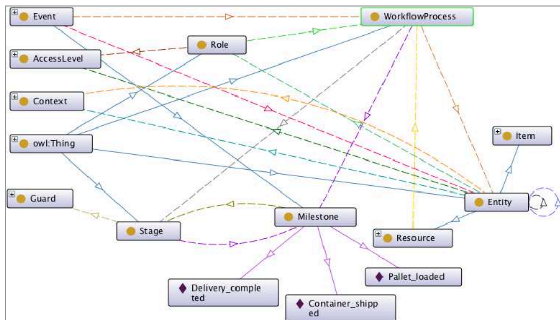
Figure 60. Ontologie du workflowProcess
