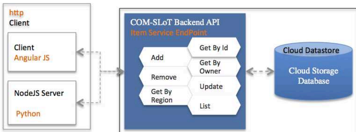
Figure 90. Service de publication des Items
