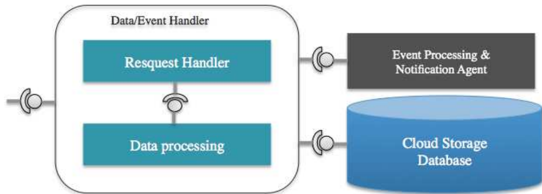
Figure 70. Architecture du composant Data/Event handler
