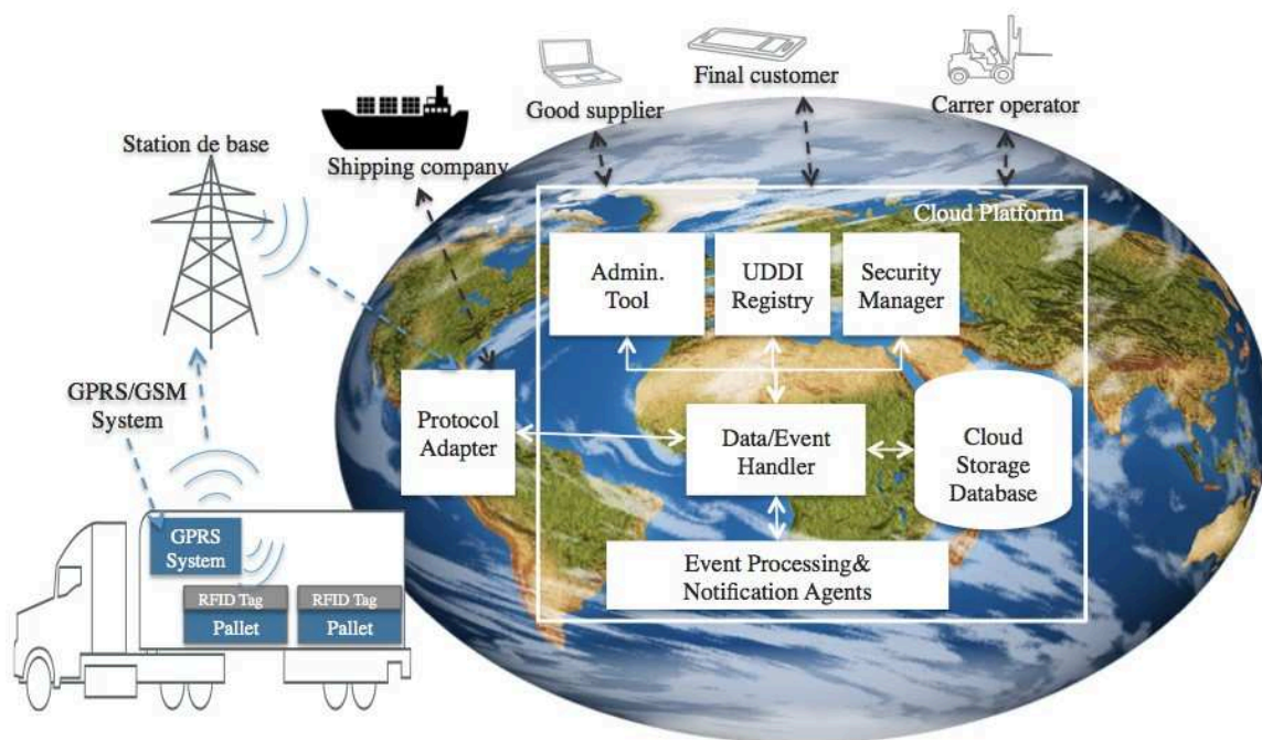
Figure 67. Architecture globale de la plateforme collaborative
