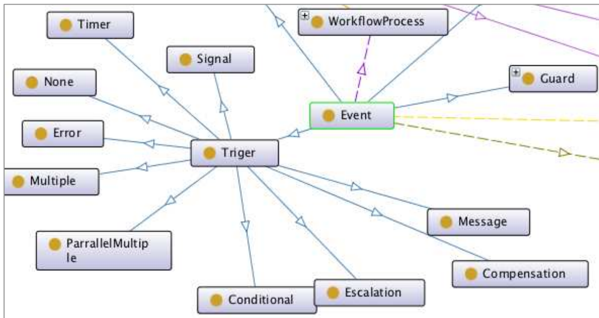
Figure 63. Ontologie des Triggers
