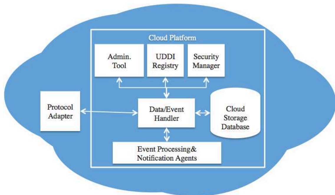
Figure 69. Architecture de la plateforme de stockage Cloud
