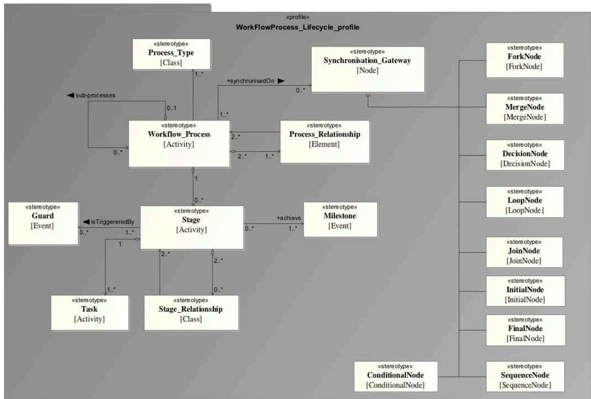
Figure 17. Profil UML des Workflow Process
