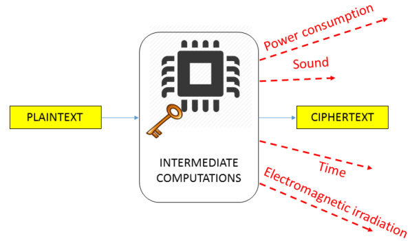
Figure 1.2: The different side channels encountered by an electronic device. Courtesy of Eleonora Cagli.
