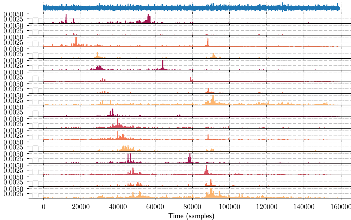
Figure 7.12: GV for one trace of the AES 8-bit implementation. The top plot depicts the considered trace, whereas the bottom plots denote the gradients for each targeted byte.
