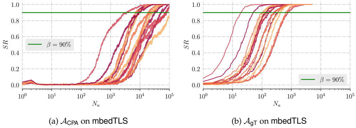
Figure 6.3: Success Rate with respect to the number of attack traces. Attacks on mbedTLS requiring the alignments of the P.o.Is. The different colors denote the different targeted bytes.
