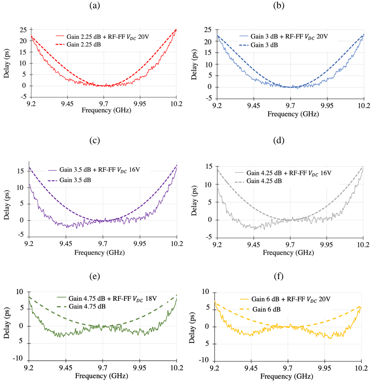
Figure 4.20 Normalized delay response of SOA-XN with (solid line) and without (dashed line) the hybrid correction structure for different gains (a)-(f).
