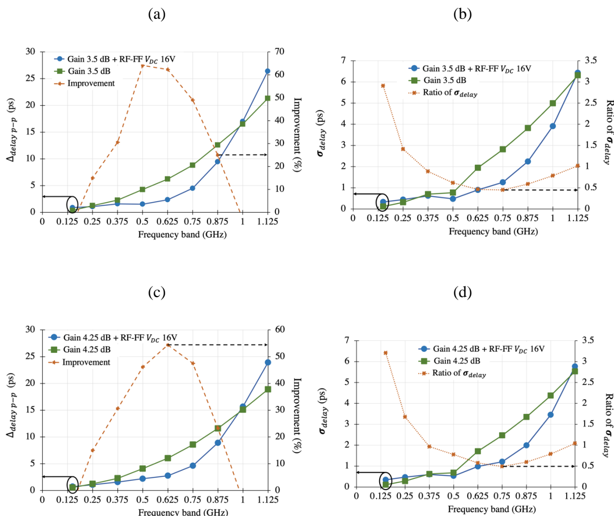
Figure 4.23 Results of second category for: \Delta_{delay p-p} and % of improvement (a) and (c). \sigma_{delay} and the ratio of \sigma_{delay} (b) and (d).
