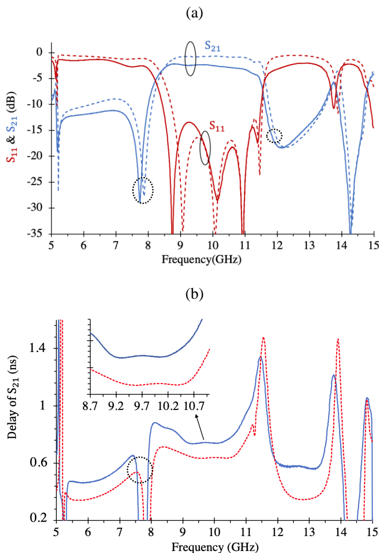
Figure 4.3 S_{11} and S_{21} of RF-FF for V_{DC} = 16V (a). Delay of RF-FF for V_{DC} = 16V (b). Simulated results (dashed lines) and measured results (solid lines).
