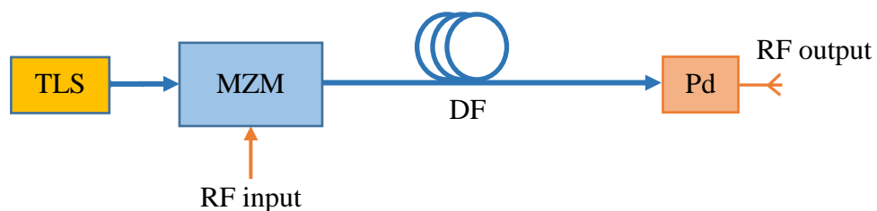
Figure 1.10 Tunable MWP delay line structure by using a length of DF.
