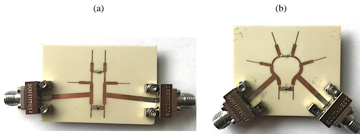
Figure 4.1 photograph of (a) RF-FF, (b) RF-CF.
