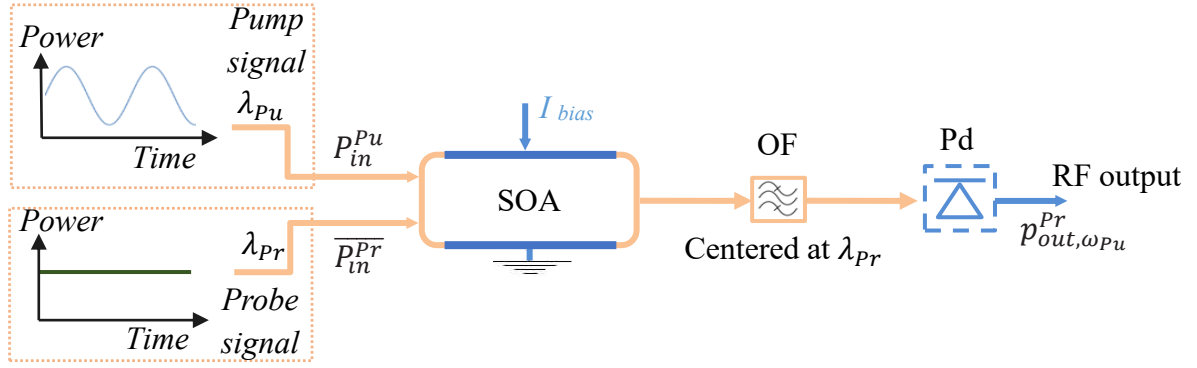
Figure 2.27 Pump-probe setup, OF: Optical filter, Pd: Photodiode.
