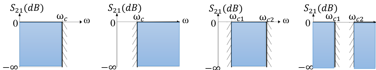
Figure 3.5 Idealized filter responses: (a) Low-pass, (b) High-pass, (c) Bandpass, and (d) notch.
