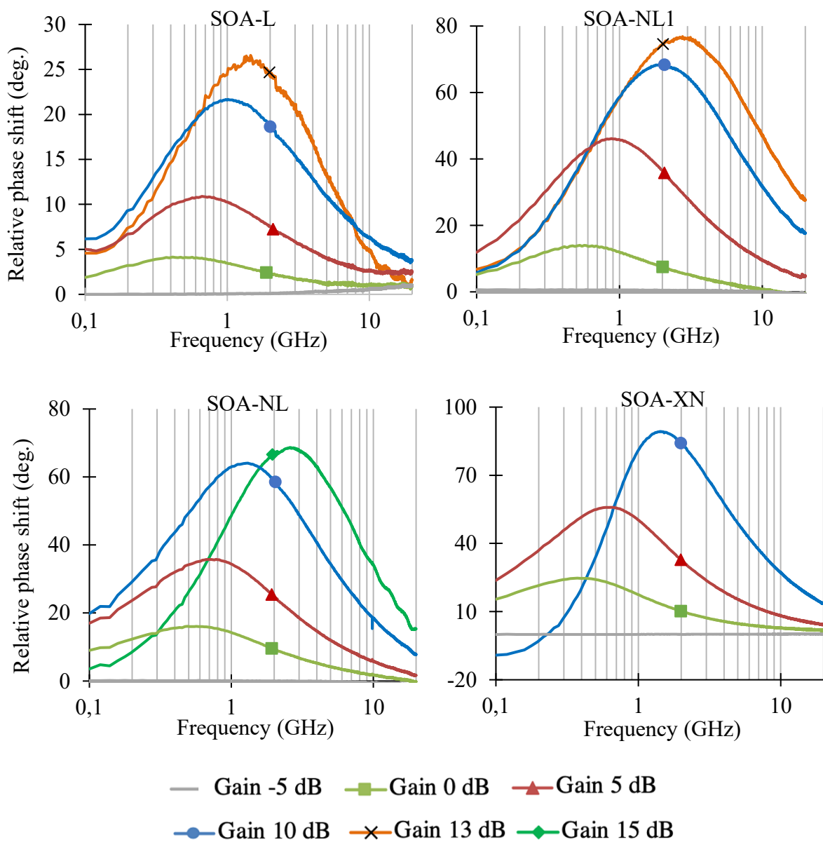
Figure 2.11 Measured relative phase shift as function of the frequency for different optical gains.
