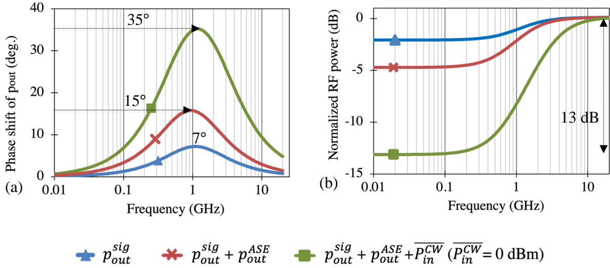
Figure 2.17 (a) Theoretical phase shift and (b) Normalized RF power of p_{out} as function of the frequency for \overline{P_{in}^{sig}} = -15 dBm and \overline{P_{in}^{CW}} = 0 dBm in presence of the ASE.
