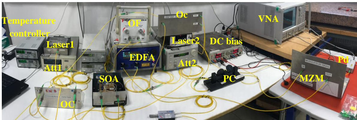
Figure 2.20 Experimental set-up.
