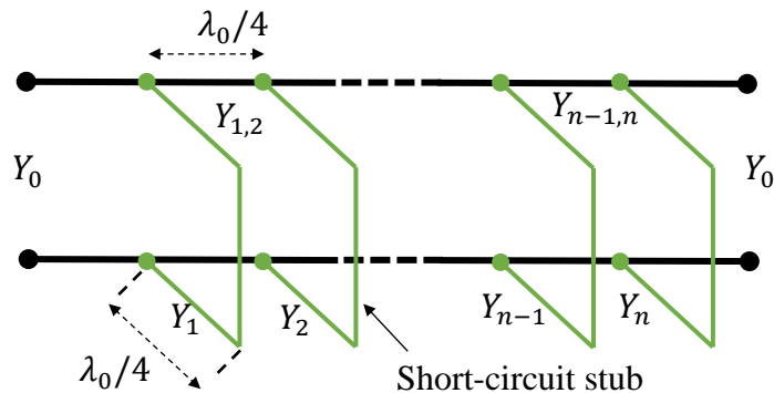
Figure 3.11 General circuit model of quarter-wavelength shunt short-circuited stubs.
