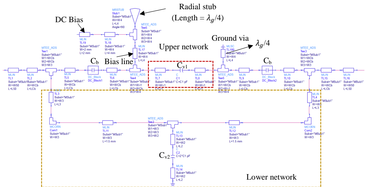
Figure 3.30 Schematic of the proposed tunable RF-PS.
