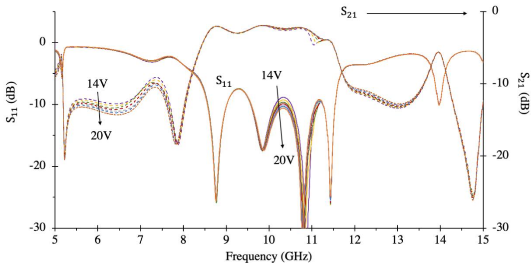
Figure 4.6 Measurement of RF-CF S_{11} and S_{21} .
