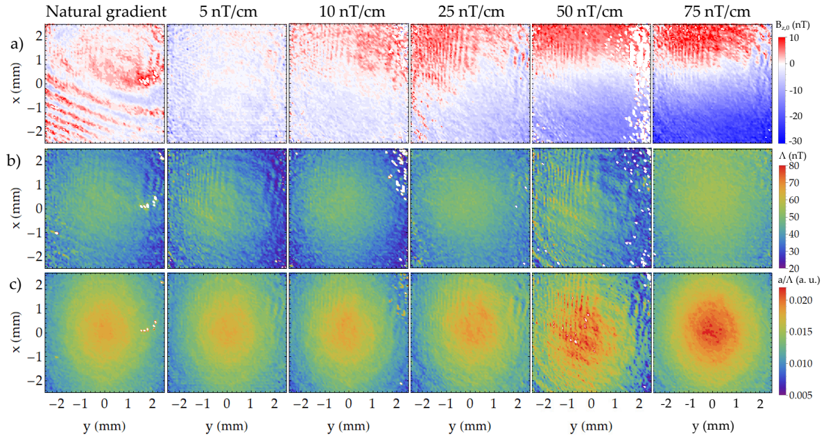
Figure 5.9: Spatial dependence of the Hanle resonances fitted offset field B_{z,0} (a) , HWHM \Lambda (b) , and amplitudes a/\Lambda (c) for several \partial B_z/\partial x gradient amplitudes. From the left column to the right column: natural gradient of the magnetic shield, \partial B_z/\partial x = 5, 10, 25, 50, 75 nT/cm. The scattering in the data for \partial B_z/\partial x = 50 nT/cm at y > 1 mm comes from failed fits due to the low Hanle resonances SNR.
