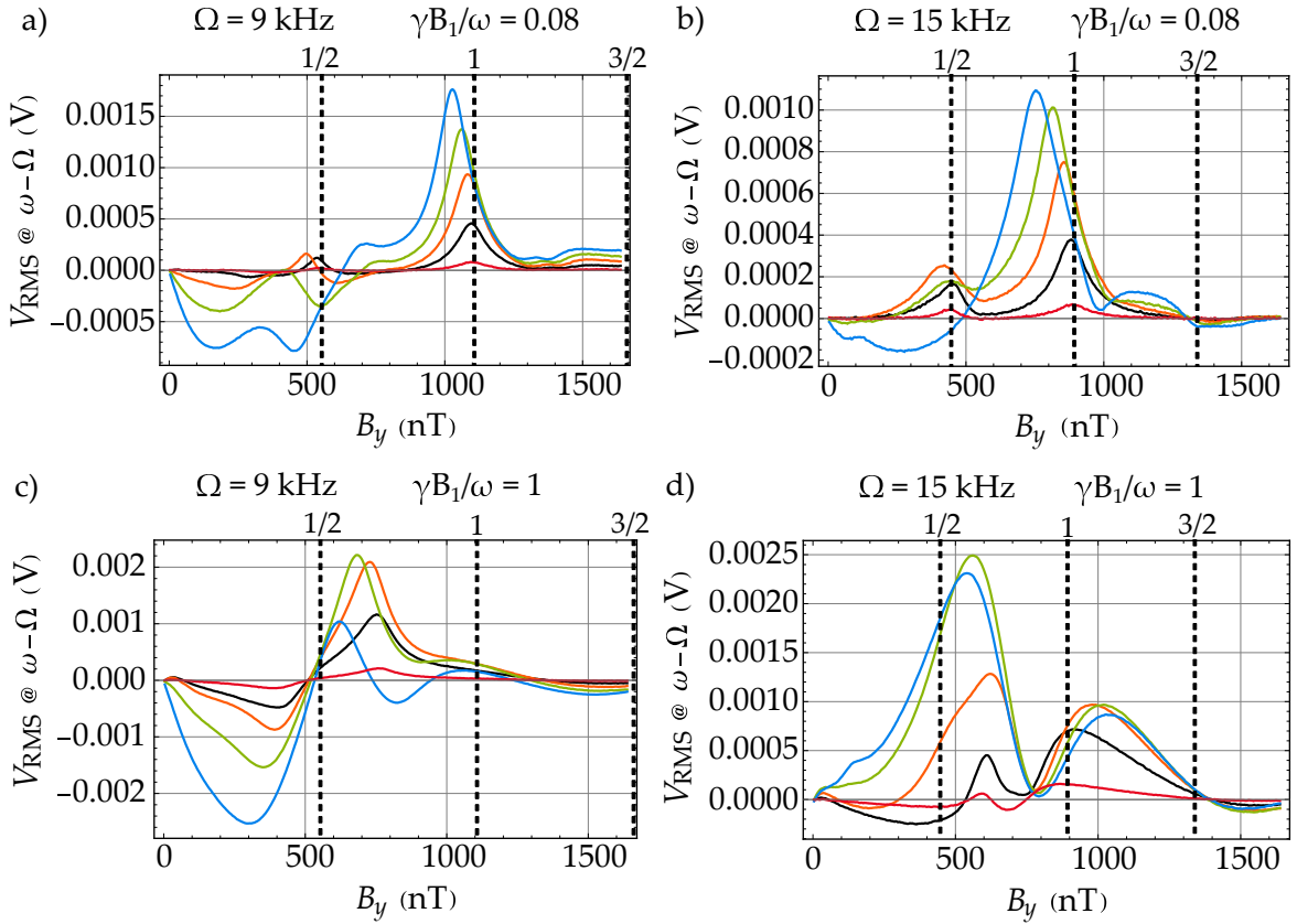
Figure 4.18: Demodulated in-quadrature signal as a function of B_y for different values of B_2 . (a) & (b) Signals at \gamma B_1/\omega = 0.08 ( \Leftrightarrow B_1 = 115.6 \text{ nT}_p ) at \Omega/2\pi = 9 and 15 \text{ kHz} respectively, for B_2 = 21.4 \text{ nT}_p (red), 124.1 \text{ nT}_p (black), 261.1 \text{ nT}_p (orange), 398 \text{ nT}_p (green) and 535 \text{ nT}_p (blue). (c) & (d) Signals at \gamma B_1/\omega = 1 ( \Leftrightarrow B_1 = 1434 \text{ nT}_p ) at \Omega/2\pi = 9 and 15 \text{ kHz} respectively, for B_2 = 21.4 \text{ nT}_p (red), 124.1 \text{ nT}_p (black), 261.1 \text{ nT}_p (orange), 398 \text{ nT}_p (green) and 535 \text{ nT}_p (blue). The vertical dashed lines show the multiples of (\omega - \Omega)/\gamma in each case.
