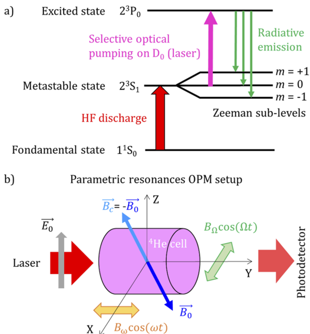
FIG. 1. (a) Simplified principle of operation of the ^4\text{He} OPM: the energy diagram describing the optical pumping process (b) and main elements of the parametric resonance magnetometer architecture.
