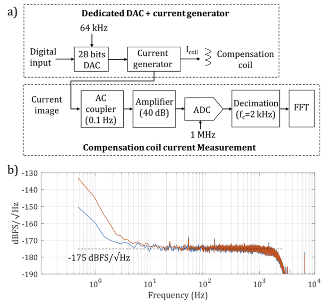
FIG. 4. Noise level performance of the compensation currents delivered by the DAC and current generator assembly in the feedback of the ^4\text{He} magnetometer closed-loop architecture: characterization method (a) and noise measurements in dB Full Scale per square root of Hertz (dBFS/ \sqrt{\text{Hz}} ) (b). In (b), the blue spectrum corresponds to a null compensation current and the orange one corresponds to a compensation current close to the full scale, i.e., equivalent to a \pm 70 \mu\text{T} magnetic field compensation.
