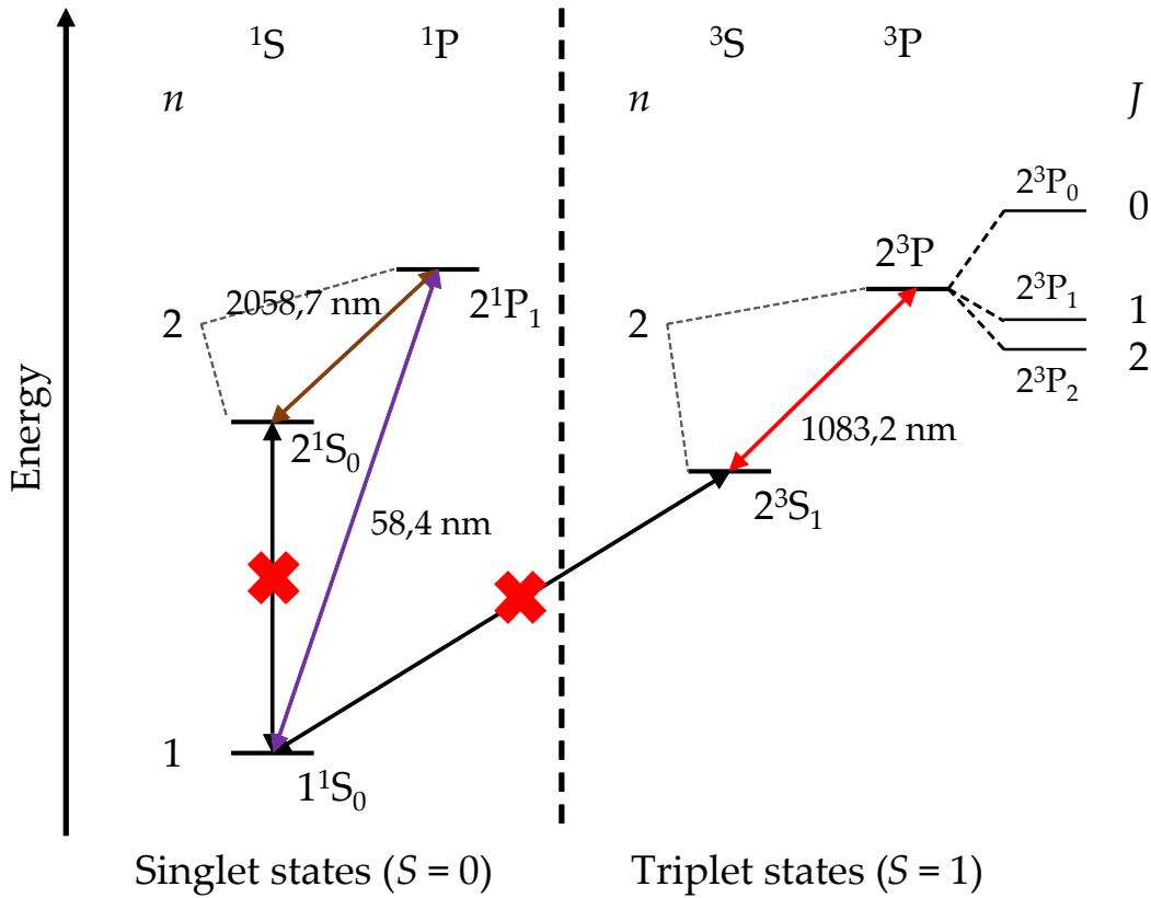
Figure 2.1: Energy level structure of {}^4\text{He} limited to the 1s2p configuration. The energy axis is not to scale. The colored arrows show the allowed E_1 transitions. The black arrows with red cross show the forbidden E_1 transition between the ground state and the two metastable states. The fine structure of the 2^3P level is shown. n corresponds to the outer electron principal quantum number for the configuration 1snl . The E_1 transition wavelengths are in vacuum standard from the reference [33].
