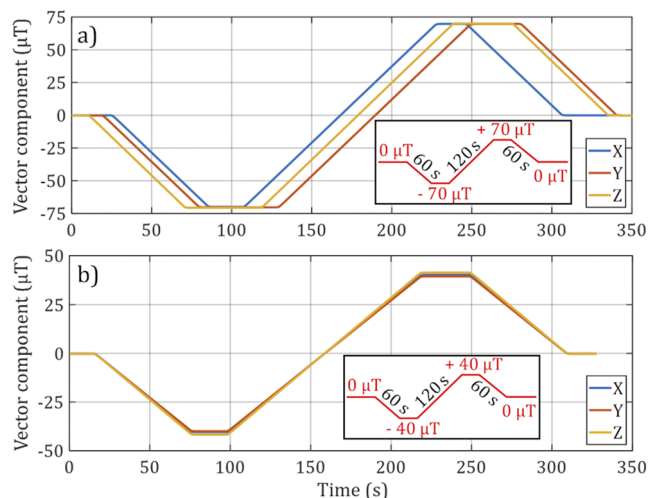
FIG. 8. Sensor measurement range verification. (a) Vector components ( \mu\text{T} ) measured during the magnetic field sweeps of \pm 70 \mu\text{T} successively performed on each axis. The inset shows the field pattern applied to the magnetometer on each axis successively (the magnetic field is set to 0 nT on the non-excited axes). (b) Vector components ( \mu\text{T} ) measured during an intercardinal magnetic field sweep of \pm 40 \mu\text{T} ( 70 \mu\text{T} max total field intensity). The inset shows the intercardinal magnetic field pattern applied simultaneously on each axis of the magnetometer.
