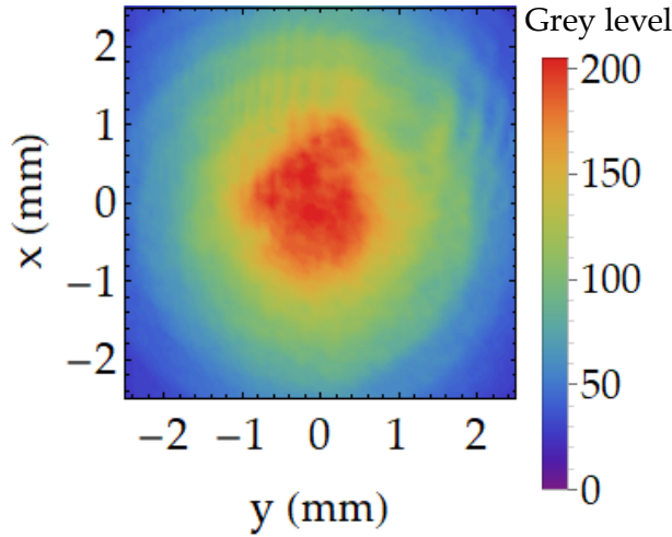
Figure 5.11: Light intensity distribution over the mapped area when the plasma is off.
