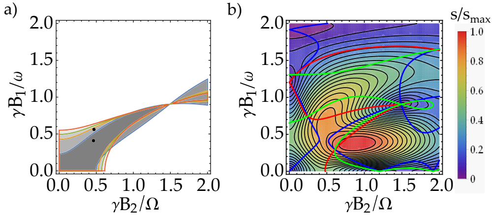
Figure 3.10: RF field amplitudes for which the non-secular contribution to the slope is higher than the secular one and theoretical dependence of the parameter s as a function of the RF fields amplitudes. (a) Areas where the non-secular contribution to the slope s_x is higher than the secular one as a function of the RF field amplitudes, for four different optical powers: 1 mW (blue border), 200 \mu W (orange border), 80 \mu W (green border) and 5 \mu W (red border). The black dots show the two RF amplitudes settings usually used: \gamma B_1/\omega = 0.41 and \gamma B_2/\Omega = 0.46 (lower one) and \gamma B_1/\omega = 0.56 and \gamma B_2/\Omega = 0.47 (upper one). The slopes are estimated using equations C.36 and C.40. The parameters for estimations are the same as in figure 3.6, without the considering double-pass in the cell. (b) Theoretical dependence of the parameter s = \sqrt{s_z^2 + s_y^2 + s_x^2} as a function of the RF field amplitudes. It is estimated for an optical power of P_{in} = 1.4 mW and RF fields with \omega/2\pi = 40 kHz and \Omega/2\pi = 9 kHz with the same parameters as in figure 3.6 without considering double-pass in the cell. The solid lines show iso-slopes between each axes (blue s_z = s_y , red s_z = s_x and green s_y = s_x ). The interesting crossing point lies at \gamma B_1/\omega = 0.29 , \gamma B_2/\Omega = 0.61 . For each point the slope \theta is optimized so that it maximizes {}^{(0)}\Delta I_{\Omega, \omega \pm \Omega} \cos(\theta) + {}^{(1)}\Delta I_{\Omega, \omega \pm \Omega} \sin(\theta) .
