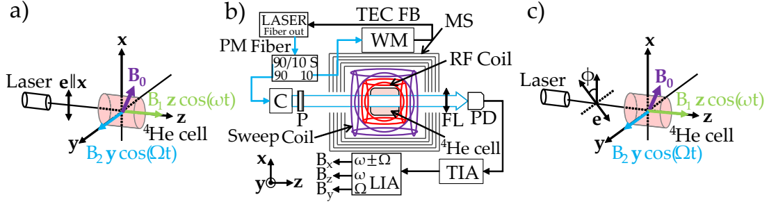
Figure 3.4: Geometry and experimental setup of the usual alignment-based PRM. (a) Geometry of the usual alignment-based PRM with pumping using linearly-polarized light of polarization \vec{e} parallel to \vec{x} and two RF fields applied in the transverse directions. (b) Experimental setup of the alignment PRM. PM: Polarization maintaining fiber; TEC FB: Thermo-Electric Controller (TEC) Feedback for laser wavelength locking; WM: Wavelength-Meter; MS: Magnetic Shield; 90/10 S: 90/10 Splitter; C: Collimator; P: Linear Polarizer; FL: Focusing Lens; PD: InGaAs Photodiode; TIA: Transimpedance Amplifier (TIA); LIA: Lock-In Amplifier. The blue paths show the optical paths and the black ones the electrical signal paths. The functions generators generating the RF fields and reference signals for the lock-in amplifier are not shown. (c) Geometry considered for the study of alignment-based PRM with linearly-polarized light which polarization \vec{e} forms an angle \phi with the \vec{x} axis and two RF fields along \vec{y} and \vec{z} .
