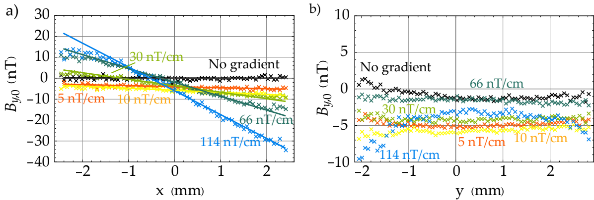
Figure 5.12: Fitted offset field B_{y,0} as a function of the position in the cell for different \partial B_y/\partial x gradient values. (a) Fitted offset field B_{y,0} as a function of the position in the cell along \vec{x} for different \partial B_y/\partial x gradient values: natural gradient of the shield (black), 5 nT/cm (orange), 10 nT/cm (yellow), 30 nT/cm (light green), 66 nT/cm (deep green), and 114 nT/cm (blue). The solid lines show the linear fits which give the following values: 0.19 nT/cm (black), 5 nT/cm (orange), 9.8 nT/cm (yellow), 31 nT/cm (light green), 66 nT/cm (deep green), and 113.7 nT/cm (blue). (b) Fitted offset field B_{y,0} as a function of the position in the cell along \vec{y} for different \partial B_y/\partial x gradient values. For both figures, the B_{z,0} values are obtained by fitting the resonance resulting from the sum of all the points over the direction transverse to the one plotted.
